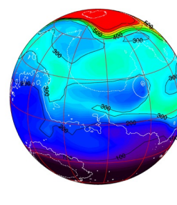
Fig. 17. Top left: map of the HDO/CO 2 volume mixing ratio, retrieved from the EXES data recorded on April 8, 2014 (Ls = 113°). Top right: GCM prediction for the same observing conditions (after Montmessin et al. 2005). Bottom left: map of the HDO/CO 2 volume mixing ratio retrieved from the TEXES data on March 1, 2014 (Ls = 96°). Bottom right: GCM prediction for the same observing conditions (Encrenaz et al. 2015).
