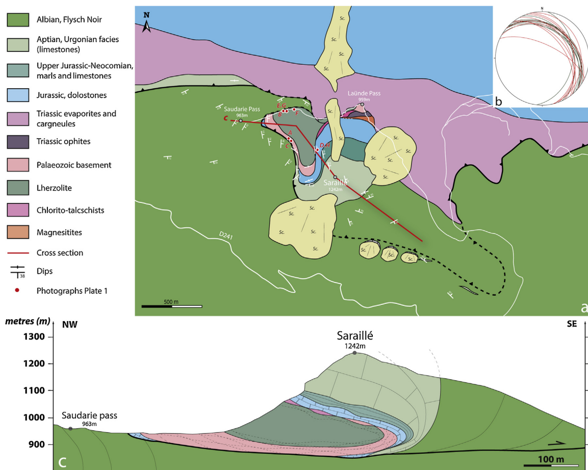
Fig. 3. a. Detailed geological map of the Saraillé massif. b. Stereogram (southern hemisphere) showing the attitude of the pyroxenitic layering in the lherzolites (green lines) and the foliation of the Palaeozoic basement (red lines) along the western boundary of the mantle body. c. NW-SE cross-section along the Saraillé massif. See Fig. 1 for location. Letters: location of photographs shown in Plate 1.
