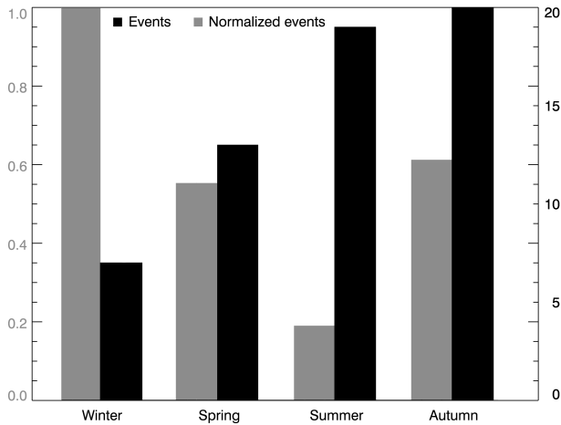
Figure 4. Seasonal distribution (black) and seasonal normalized distribution (grey) of the detected lightning–LEP events. The seasonal distribution has been normalized by the seasonal total number of lightning flashes occurring over the domain and scaled according to the winter season.
