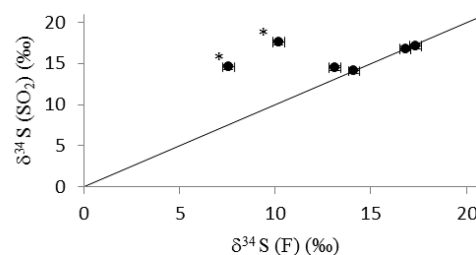
Figure 7. The isotope ratio ( \delta^{34}\text{S} value) for F_{<0.49\mu\text{m}} and \text{SO}_2 filters along with the 1 : 1 line. Two samples with different \delta^{34}\text{S} values for \text{SO}_2 and F_{<0.49\mu\text{m}} filter sulfate are shown with asterisks.
