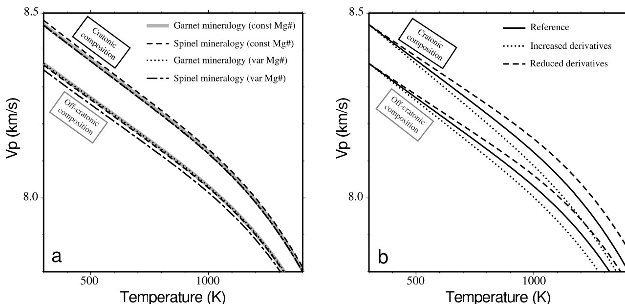
Figure 9. P wave velocity and temperature calculated for on-craton and off-craton composition (Table 4). (a) Results for two different mineralogical facies (garnet-lherzolite and spinel-lherzolite) and two models of the Fe/Mg distribution within minerals. Details of mineralogical compositions and Mg # variations are given by McDonough and Rudnick [1998]. (b) Effect of uncertainties in \partial\mu/\partial T and \partial K/\partial T for olivine. “Increased” and “reduced” derivatives correspond to the upper and lower bounds reported by Goes et al. [2000].
