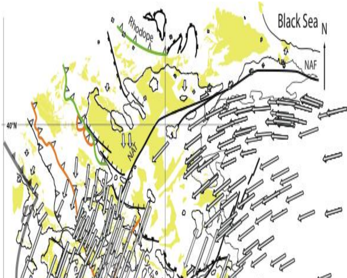
Fig. 7. Present-day displacements (after Nyst and Thatcher 2004) superposed to the map of Neogene basins (Yellow) showing that a major change occurred in the course of post-Middle Miocene deformation when the North Anatolian Fault (NAF) localized and connected to the North Aegean Through (NAT).
