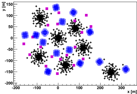
Figure 2: Central core of LOFAR. The black crosses are the low-band antennas, the blue open squares indicate the tiles of high-band antennas and the filled squares are the particle detectors.
