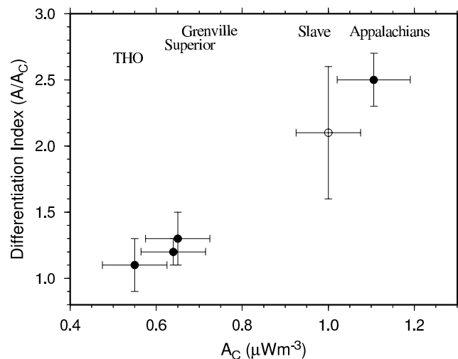
Figure 12. Differentiation index of crustal rocks ( \bar{A}/A_c ), where \bar{A} is the surface-averaged heat production and A_c is the bulk average heat production, as a function of the bulk average heat production. The Slave Province calculation is represented by an open circle since the heat flow data set is small compared to those in the other provinces. Error bars associated with D_i and A_c were calculated assuming a wide range for Moho heat flow between 12 \leq Q_M \leq 18 \text{ mW m}^{-2} .
