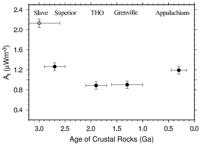
Figure 11. Average bulk crustal heat production back calculated to its value at the time of accretionary events in the given geological provinces. The Slave Province calculation is represented by an open circle since the heat flow data set is small compared to those in the other provinces. Error bars on A_t were calculated assuming a wide range for Moho heat flow between 12 \leq Q_M \leq 18 \text{ mW m}^{-2} . Error bars in x are the uncertainties in the ages of major crustal accretion events.
