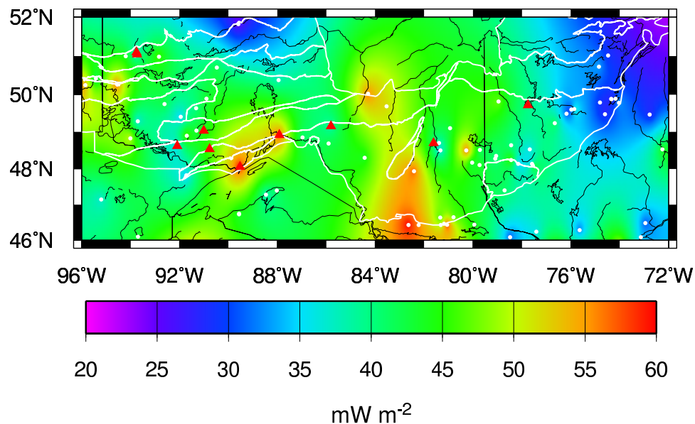
Figure 6. Heat flow in the Superior Province, with sites affected by late stage thermal perturbations removed. These sites include the Nipigon Embayment, where mafic intrusive Logan dikes resulted from the Keweenawan rifting; the Kapuskasing site where the upper crust was eroded following uplift; and the Lake Superior sites which were significantly affected by Keweenawan rifting events. Red triangles represent the new heat flow sites. White circles represent previous land heat flow measurement sites. Thin white lines mark subprovince boundaries.
