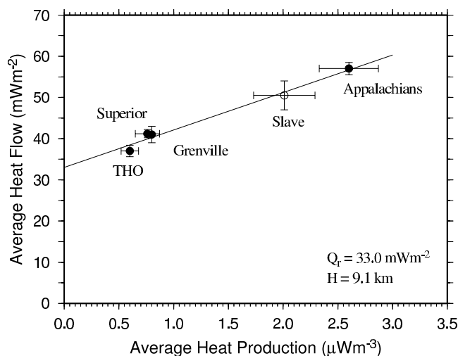
Figure 9. Mean heat flow and surface heat production in the Canadian Shield comprising averages for the Archean Slave and Superior provinces, the juvenile THO (excluding the Thompson Belt), the Grenville, and the Appalachians. The Slave Province data are represented by an open circle since the heat flow data set is small compared to those in the other provinces. Bars show the standard error on the mean. The line is the best fit to the data.
