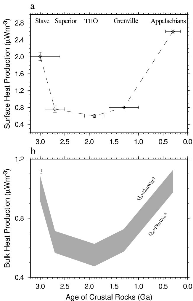
Figure 10. (a) Average surface crustal heat production as a function of ages of crustal accretion events in the Archean Slave and Superior provinces, in the Proterozoic THO and Grenville provinces, and the Paleozoic Appalachians. Error bars in y show the standard error on the mean. Bars in x are the uncertainties in the ages of major crustal accretion events. (b) Average bulk crustal heat production as a function of ages of crustal accretion events. Average bulk crustal heat production is calculated based on a large range for Moho heat flow between 12 \leq Q_M \leq 18 \text{ mW m}^{-2} . Crustal thickness, used in the calculation is based on the mean value for each region according to Perry et al. [2002]. The Slave Province bulk heat production is poorly constrained since only three heat flow sites are available.
