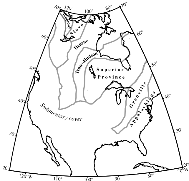
Figure 1. Generalized geological map of North America showing the Archean cratons and Proterozoic and Paleozoic orogens and provinces (modified from Hoffman [1989] ).
