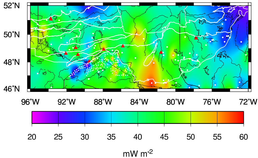
Figure 5. Heat flow in the Superior Province. Red triangles represent the new heat flow sites (summary in Table 1). Large white circles represent previous land measurements, and small circles represent lacustrine data in Lake Superior [Hart et al. , 1994]. Thin white lines mark subprovince boundaries.
