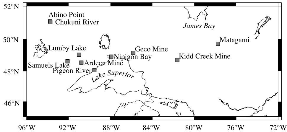
Figure 3. Locations of new heat flow sites in the Superior Province. The heat flow data are tabulated in Table 1.
