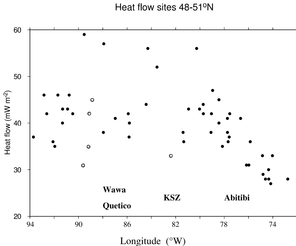
Figure 7. Longitudinal profile of the surface heat flow across the Superior Province. The open circles are heat flow values in the Nipigon Embayment and KSZ.
