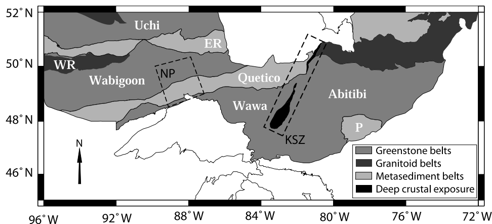
Figure 2. Generalized geological map of the Superior Province of the Canadian Shield showing major subprovinces from Card and Ciesielski [1986] and J. Percival (personal communication, 2005) . ER is the English River metasedimentary subprovince, WR is the Winnipeg River plutonic subprovince, and P is the Pontiac metasedimentary subprovince. The boxes show the location of the Nipigon Embayment (NP) and the Kapuskasing Structural Zone (KSZ).
