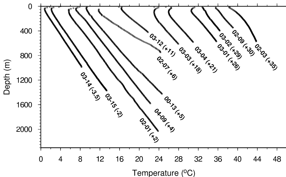
Figure 4. Temperature-depth profiles at the borehole heat flow site locations given in Table 1 (Superior Province). The profiles are shifted horizontally as indicated (in °C) to avoid superposition.
