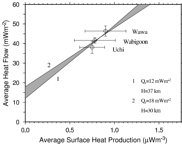
Figure 8. Mean heat flow and surface heat production in the Uchi, Wabigoon, and Wawa subprovinces of the Superior. The averages contain data presented in Table 5 where sites affected by late stage thermal perturbations have been removed. Bars show the standard error on the mean. The grey zone marks the upper and lower limits of the inferred relationship, taking a wide range of estimates for Q_M between 12 \leq Q_M \leq 18 \text{ mW m}^{-2} .
