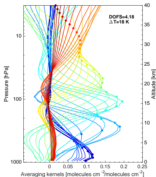
Figure 1. Example of IASI-A averaging kernel functions corresponding to one daytime midlatitude measurement ( 31.3^{\circ} N, 46.7^{\circ} E) obtained on 15 July 2014 for each 1 km retrieved layer from the surface to 40 km altitude (color scale). The total DOFS and thermal contrast are also indicated.
