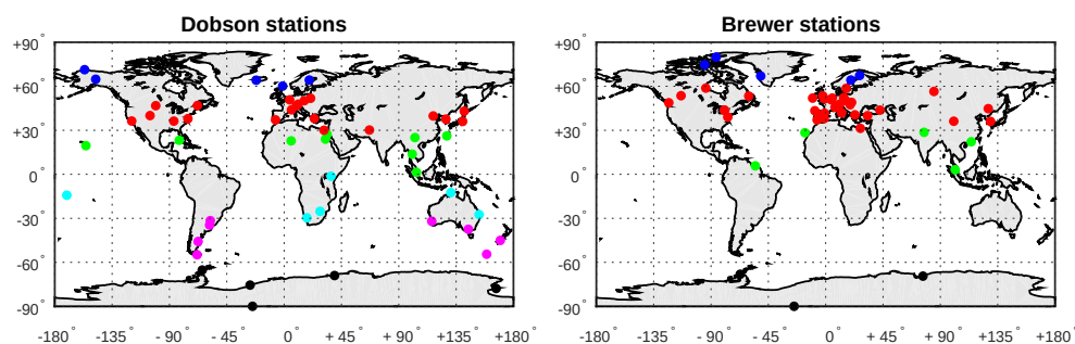
Figure 9. Location of the WUODC network of ground-based stations used in the present validation exercise; Dobson stations are shown on the left and Brewer stations on the right. The colors indicate different latitude bands: 60–90° N (blue), 30–60° N (red), 0–30° N (green), 0–30° S (cyan), 30–60° S (magenta), and 60–90° S (black).
