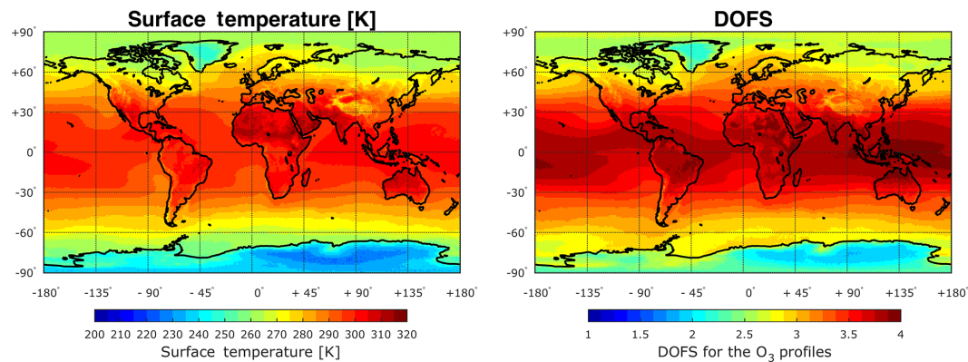
Figure 2. Global distribution averaged over 1^\circ \times 1^\circ for the period 2008–2014 for daytime measurements: (left) IASI surface temperature and (right) DOFS for the \text{O}_3 profiles.
