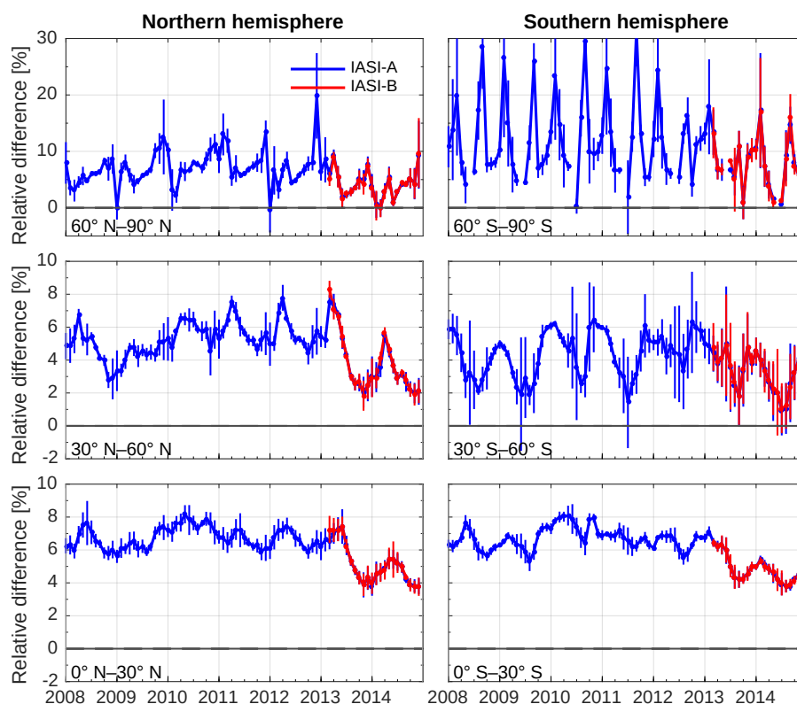
Figure 7. Time series of the monthly relative differences (in percent) between IASI-A (blue) and IASI-B (red) against GOME-2A O3M SAF total ozone columns for different latitudinal bands. The associated standard deviation is also displayed.
