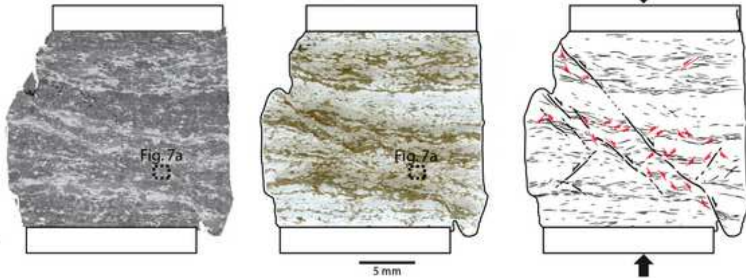
b) He/900/21-32: \dot{\gamma}=10^{-4}-10^{-3} \text{ s}^{-1} , Strain=27%, Glass=21 \pm 7 - 32 \pm 6%
