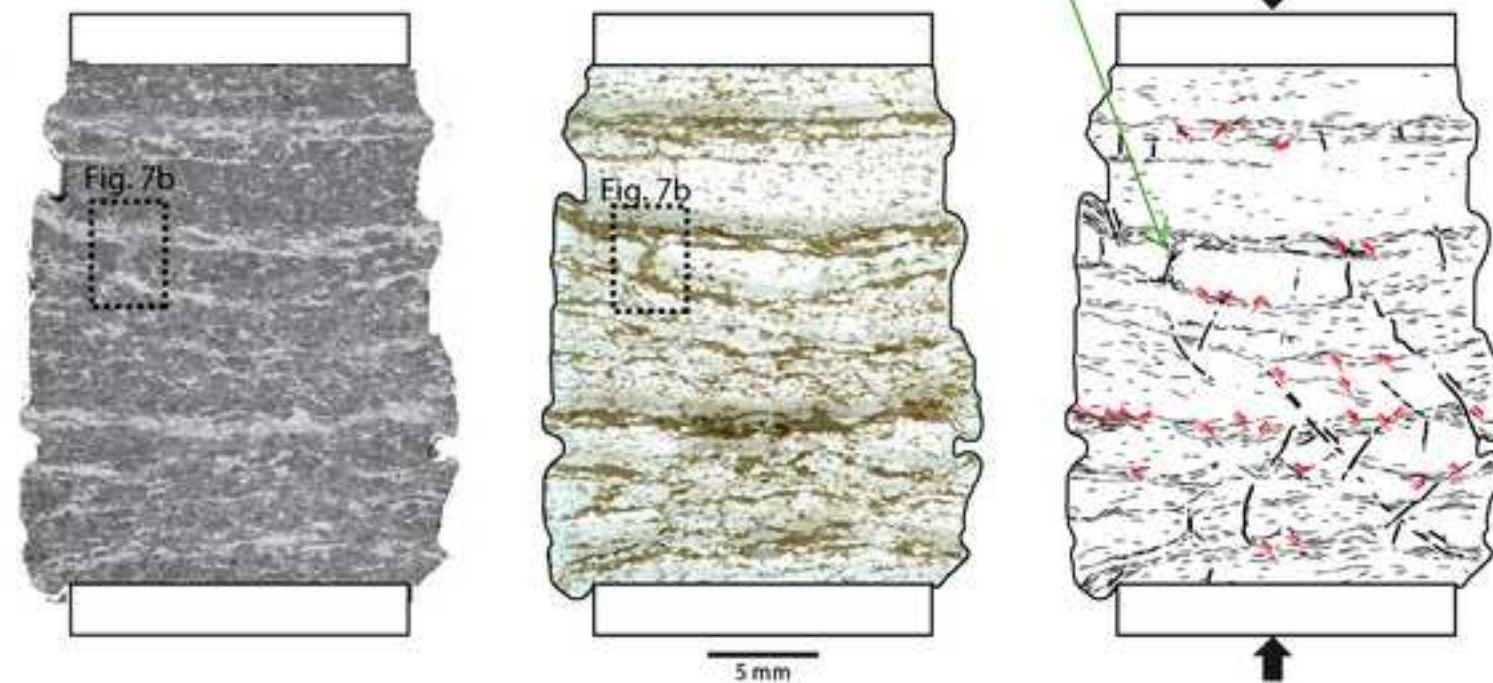
b) He/900/21-32: \dot{\gamma}=10^{-4}-10^{-3} \text{ s}^{-1} , Strain=27%, Glass=21 \pm 7 - 32 \pm 6%
