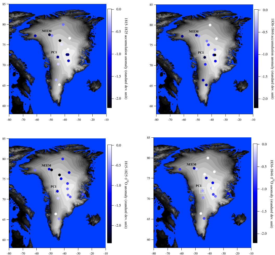
Figure 15. Map of accumulation (top) and \delta^{18}\text{O} (bottom) anomaly during 1815–1825 (left) and 1836–1846 (right) (corresponding respectively to the coldest-driest 11-year periods in PCI and NEEM), calculated from individual records, as anomalies from the 1761–1966 average, and divided by the standard deviation of 11-year averages for 1761–1966 (in standard deviation units).
