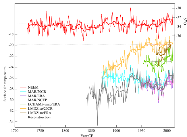
Figure 11. Comparison of NEEM δ 18 O (red, in ‰) with gridded temperature reconstructions and simulations (in °C).
