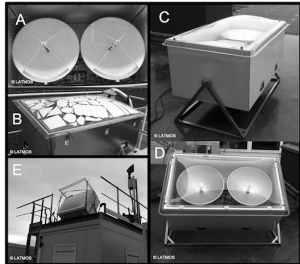
FIG. 1. Photos of the radar. (a),(b) Top view showing antennas and electronics, and the outside of the original prototype deployed at SIRTA. (c)–(e) BASTA-MOBILE in different positions.
