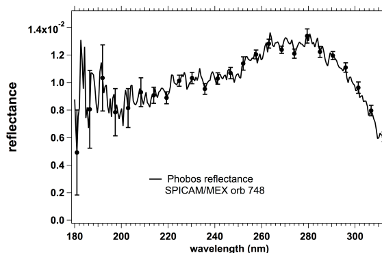
Figure 2. UV reflectance of Phobos (phase angle 22°) in the 180-312 nm range obtained by SPICAM at orbit 748. A systematic uncertainty of \pm 20\% should be added to the error bars which reflect measurements statistics.
