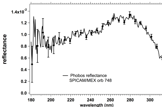
Figure 2. UV reflectance of Phobos (phase angle 22°) in the 180-312 nm range obtained by SPICAM at orbit 748. A systematic uncertainty of ± 20% should be added to the error bars which reflect measurements statistics.
