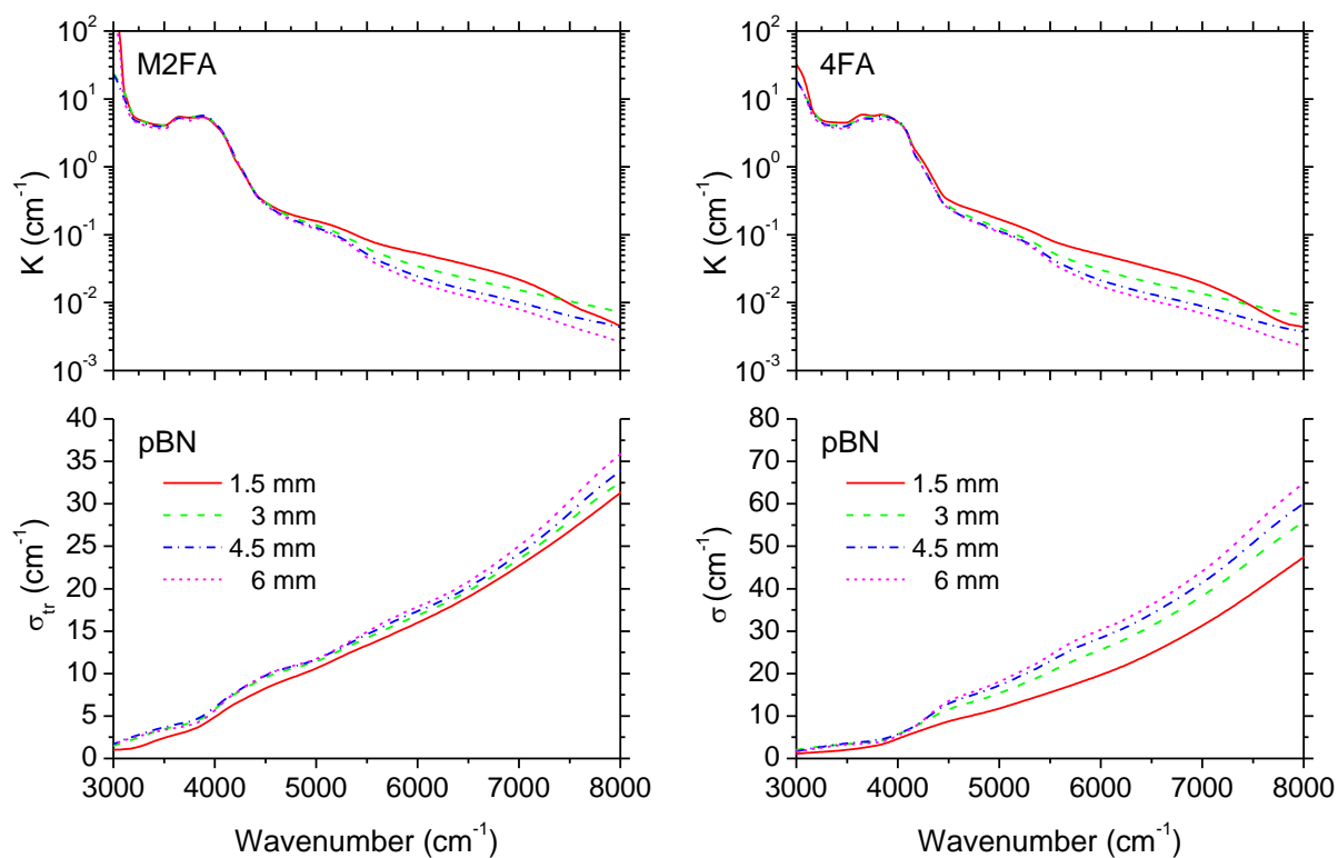
Fig. 6: Absorption and scattering coefficients of pBN-AR identified with M2FA and 4FA models for different sample thicknesses.
