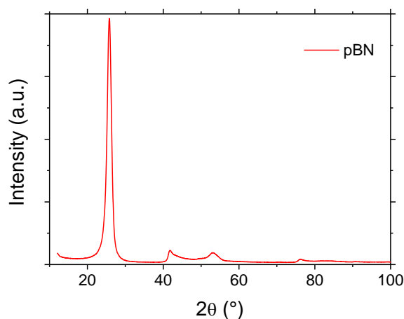
Fig. 1: X-ray diffraction pattern of pBN.
