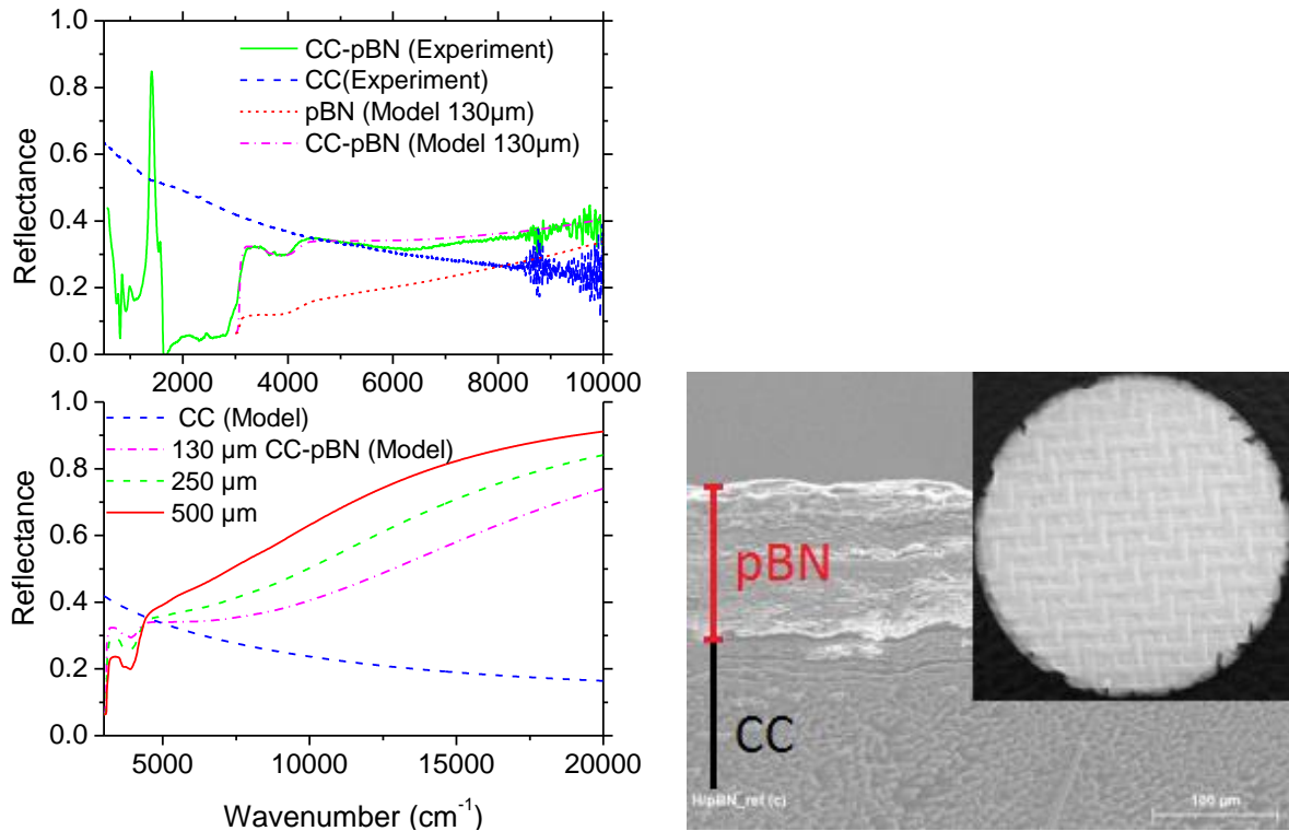
Fig. 7: Normal hemispherical reflectance spectra of carbon-carbon composite (CC) and of carbon-carbon composite coated with 130µm of pBN (CC-pBN). Estimations of the reflectance of coated carbon-carbon composite with increasing thicknesses obtained with Eq. (10) are displayed in the lower part of the figure.
