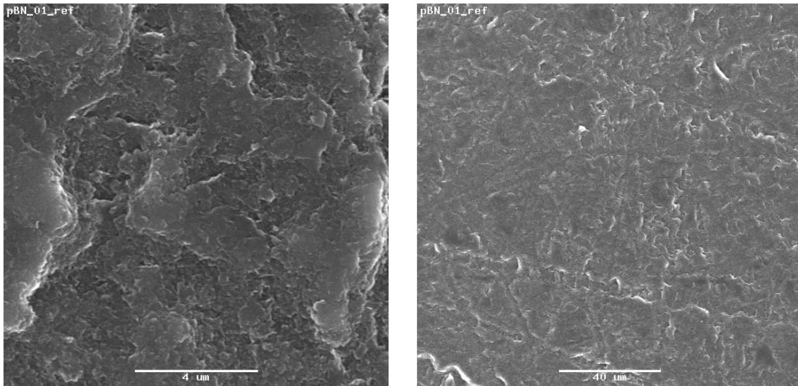
Fig. 2: SEM images of the pBN surface, scale bars: on the left 4 \mu m and on the right 40 \mu m
