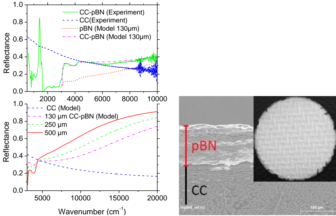
Fig. 7: Normal hemispherical reflectance spectra of carbon-carbon composite (CC) and of carbon-carbon composite coated with 130 \mu m of pBN (CC-pBN). Estimations of the reflectance of coated carbon-carbon composite with increasing thicknesses obtained with Eq. (10) are displayed in the lower part of the figure.
