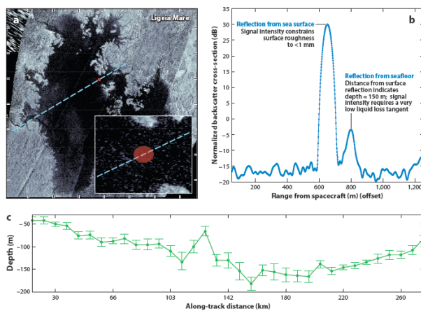
Figure 1: RADAR sounding measurements over Ligeia Mare. (a) A Synthetic Aperture Radar (SAR) mosaic of Ligeia Mare with the position of the May 2013 (flyby T91) altimetry track highlighted and the location of an example altimetry echo shown on the right. (b) An example of a double-peaked waveform observed over Ligeia, with returns from the sea surface and seabed labeled. (c) The along-track bathymetry derived by Mastrogiuseppe et al. [4,5].
