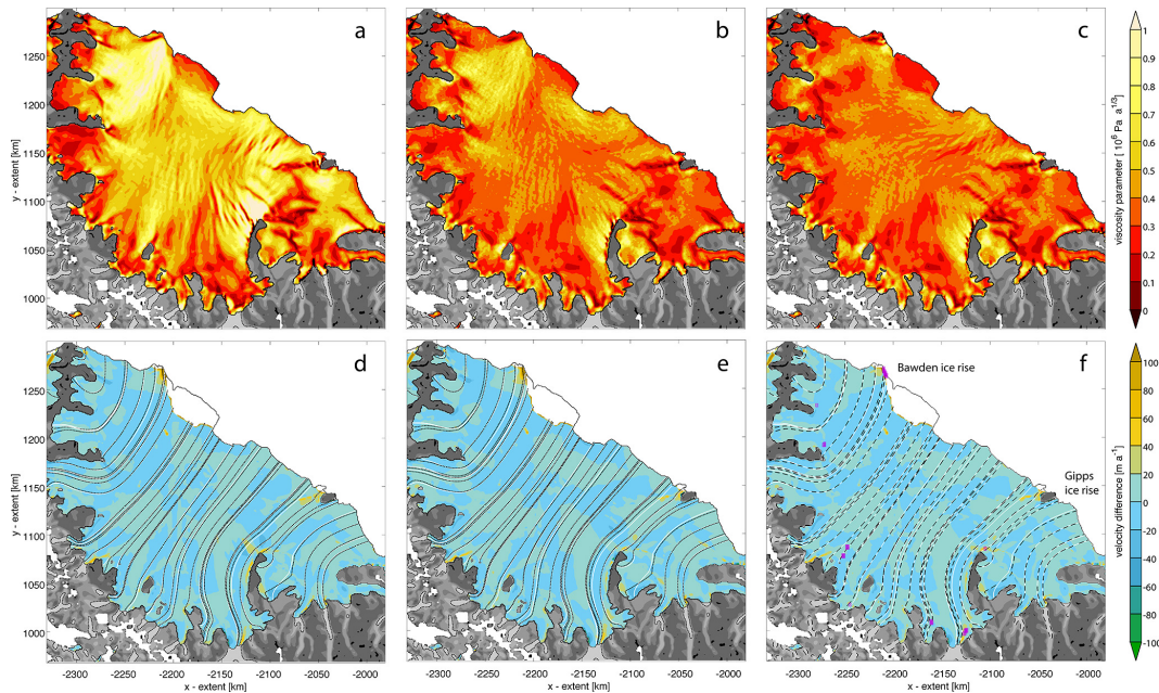
Figure 3. Ice viscosity parameter ( a–c ) as inferred by the control method for the Larsen C Ice Shelf. Velocity difference ( d–f ) as in Fig. 1. Panels ( a, d ) show results based on the actual Bedmap2 geometry, while panels ( b, e ) show results after flotation is guaranteed using the \mathbb{T} method. Inversion results on Larsen C for the \mathbb{T} geometry accounting for friction beneath pinning points not included in Bedmap2 ( c, f ). Grey shading indicates observed velocity magnitude on grounded parts of the ice sheet. The Bedmap2 shelf extent is indicated by a black contour line. On the shelf, black dashed and white lines indicate observed and modelled streamlines respectively. The black dashed line on the grounded areas gives the 100 \text{ m a}^{-1} isoline of the observed surface velocities. Locations of pinning points (PIN5) not in Bedmap2 are indicated with pink squares in panel ( e ).
