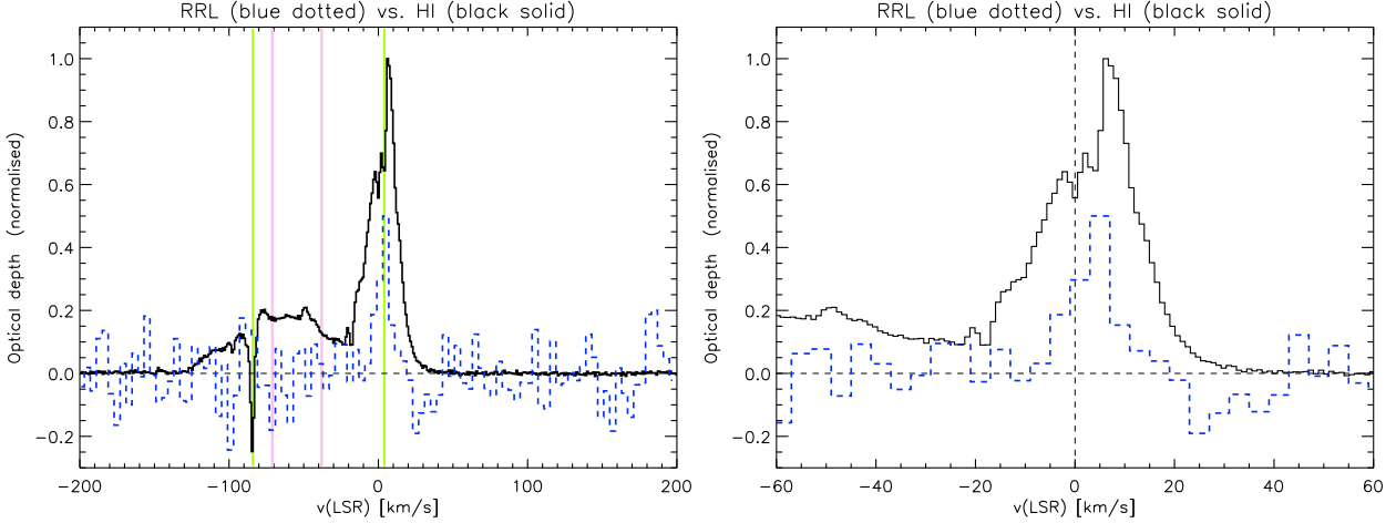
Figure 3. Comparison of the foreground ( z = 0 ) stacked carbon \alpha absorption with the HI emission along the line of sight to Cyg A. The HI emission, from the LAB survey (Kalberla et al. 2005), is given by the black line. The inverted carbon \alpha absorption (this work) is shown by the dashed blue line. For clarity the HI emission has been normalised to 1.0 and the inverted RRL absorption has been normalised to 0.5. ( Left ) HI and RRL in the velocity range \pm 200 \text{ km s}^{-1} . The vertical green (CNM) and purple (WNM) lines show the positions of the strongest HI 21 cm components observed in absorption towards Cyg A (Carilli et al. 1998). ( Right ) The central \pm 60 \text{ km s}^{-1} range.
