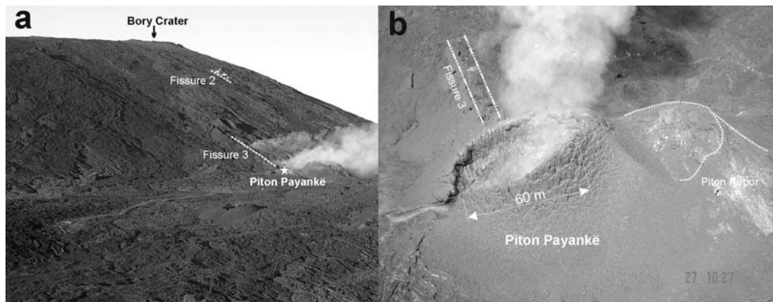
Figure 2. (a) View of the northern flank of Piton de la Fournaise on 23 August 2003. The star at the base of the third fissure indicates the location of Piton Payanké. On its right is visible the Piton Kapor, the main cone of the 1998 eruption; (b) By 27 August, Piton Payanké has grown over Piton Kapor (photos by Th. Staudacher).
