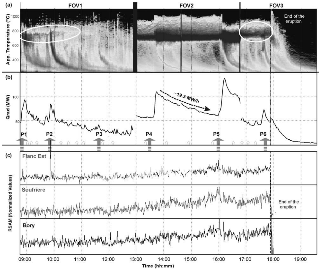
Figure 13. Synthesis of thermal data recorded on 27 August 2003, compared with seismic records (a) “RadTherm” of the whole sequence; (b) Radiative heat flux ( Q_{\text{Rad}} ) derived from the “RadTherm”; major peaks correspond to the occurrence of pulses episodes. The roofing process causes a marked decrease in the heat radiated by the flow surface; (c) RSAM (1 min) recorded at three seismic stations (data provided by the Observatoire Volcanologique du Piton de la Fournaise).
