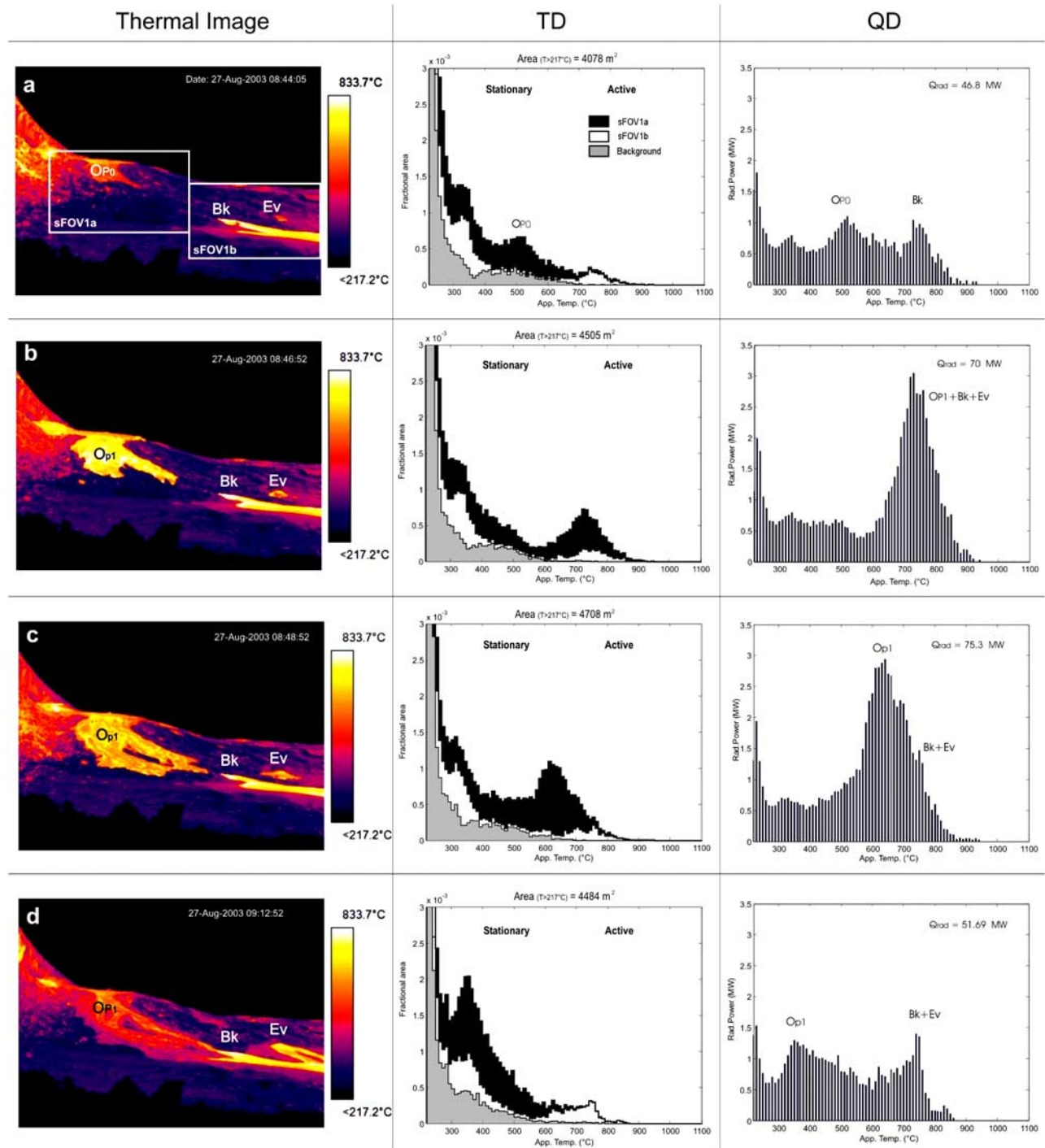
Figure 10. Thermal images, TD, and QD during the pulse P1: (a) before the pulse two main components represents a older lava pond overflow ( OP_0 ) and the active Bk; (b) P1 generates a new overflow ( OP_1 ) and the opening of Ev, whose thermal components overlap the Bk component in the active region; (c) once the pulse ceased, the overflow cools and its component “move” toward the stationary region. The Bk and Ev components are persisting in the active region; (d) the overflow cooled down (its component is being absorbed by the background), and the Bk and Ev components have increased their activity.
