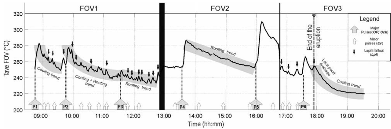
Figure 7. Time series for the FOV's average temperature. Major pulses (P1 to P6) produced clear thermal anomalies because of lava pond overflows, channel overflows, and formation of ephemeral vents. Two different trend of decreasing temperature may be distinguished, the nonlinear decrease is associated to cooling, and the linear decrease is due to the roofing process.
