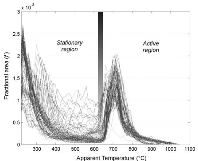
Figure 9. Overlapping of the TD for the whole sequence of images. Two distinct sectors can be observed, the lower temperature region represents “stationary” surfaces that cools within the FOV whereas the high-temperature region represents “active” lava surfaces that are moving. The transition between the two zones occur at about 630 ^{\circ}\text{C} .
