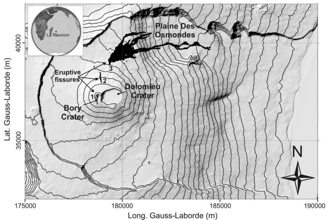
Figure 1. Location of the August 2003 eruption. The first fissure opened within the Bory Crater and was followed by two more fissures on the northern flank of the volcano. The northernmost fissure produced a 5-km long lava field within five days of activity.
