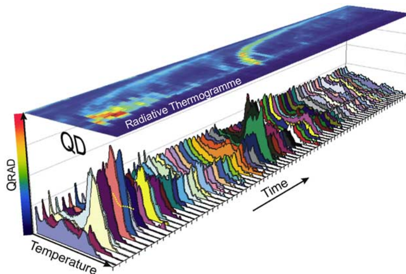
Figure 11. Three-dimensional image for the construction of the radiative thermogramme (named “RadTherm”) The QD are placed side by side and their intensity is represented according to a logarithmic color scale of the radiative heat flux ( Q_{\text{Rad}} ).
