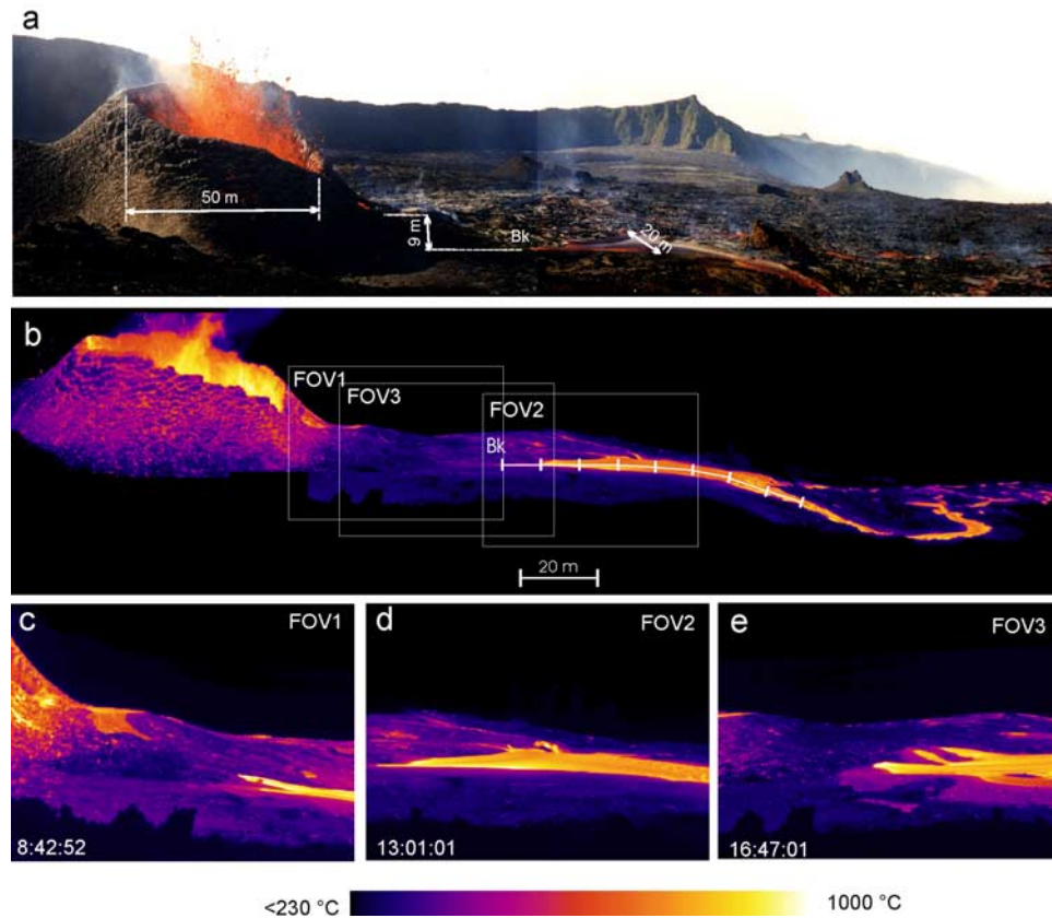
Figure 5. (a) Optical image of the vent area, the lava is flowing through Bk into the main lava channel that is forming the lava field; (b) Thermal image of the vent area, three different FOV describe the activity at the base of Piton Payanké; (c) FOV1 started on 27 August 2003 at 08:42:52 and was focused on the lava pond's overflows and ephemeral vents; (d) FOV2 started at 13:01:01 and was focused on the activity within the channel; (e) FOV3 started at 16:47:01 and was again focused on the pond's overflows and ephemeral vents.
