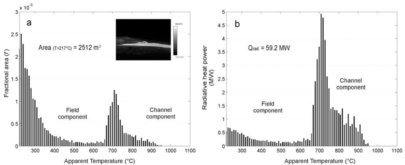
Figure 8. (a) TD of the image collected at 13:01:01. Main components are related to channel surface, and adjacent lava field; (b) Radiative heat power distribution (QD) of the cited image. The channel component is much more evident because of the higher temperature of its surface.
