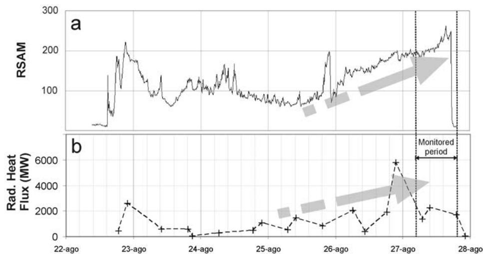
Figure 3. Seismic and thermal activity during the eruption. (a) RSAM recorded by the “La Soufriere” seismic station showing the increasing trend in tremor amplitude during the last days of eruption; (b) Radiative heat flux calculated from the MODVOLC data, following Wright et al. [2004]. Seismic data were provided by the Observatoire Volcanologique du Piton de la Fournaise; MODIS data were provided by HIGP-MODIS Thermal Alert Team.
