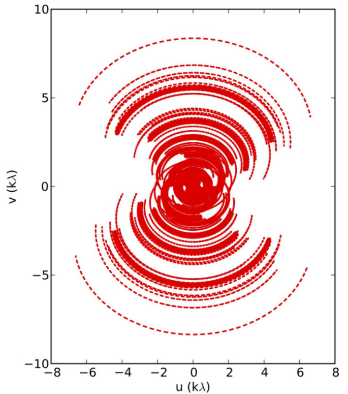
Figure 1. UV coverage of the 3C 295 observations. The relatively large fractional bandwidth fills the uv plane radially (not shown in the figure).
