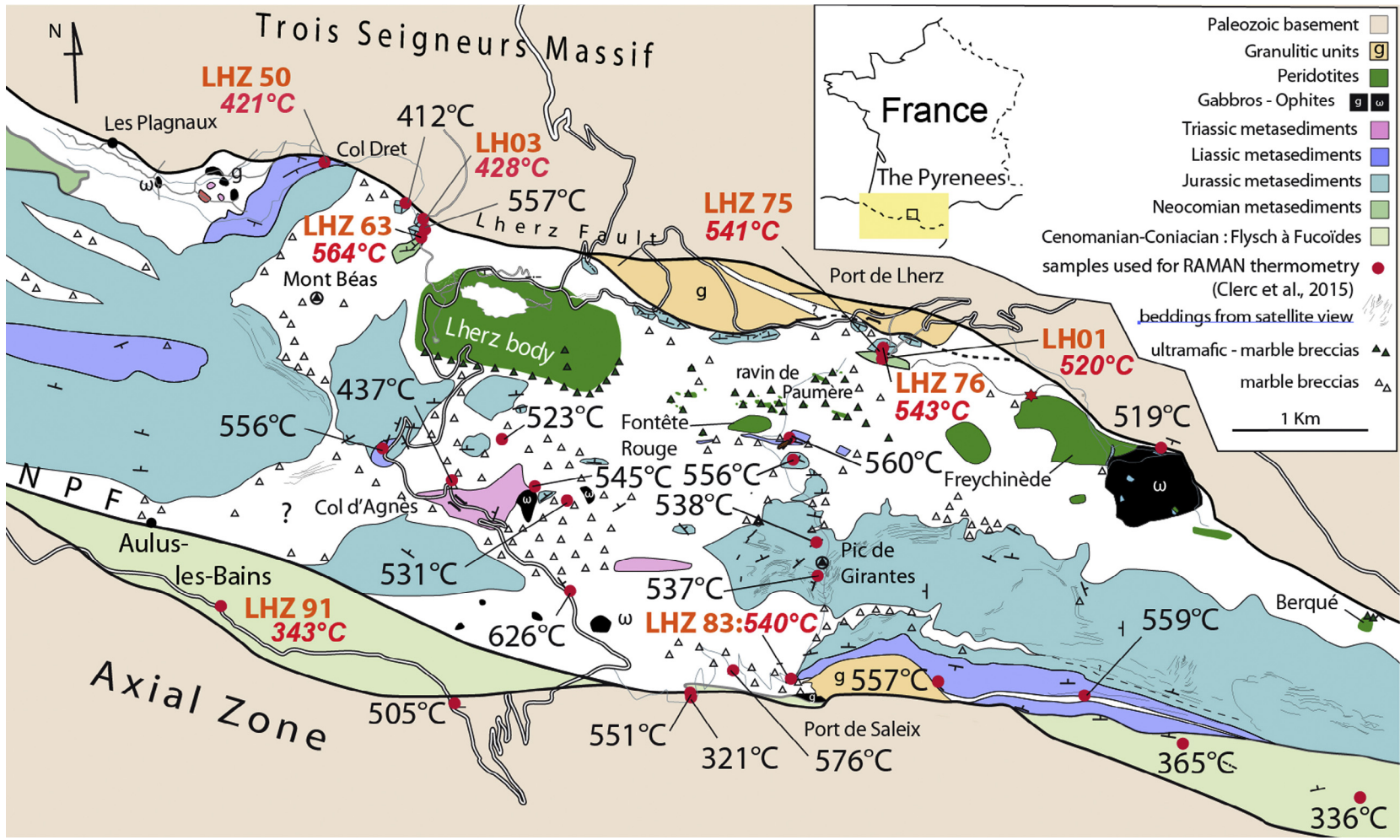
Fig. 1. Geological map of the central part of the Aulus basin based on unpublished field data collected by Y. Lagabrieulle (2006–2009) and during the Master and PhD works by C. Clerc (2008–2012). Units of massive carbonates are separated by wide areas of polymictic sedimentary breccias. The ultramafic-bearing breccias are restricted to the central part of the Aulus basin where the peridotite bodies are concentrated. Samples used for CPO calculations are reported (bold orange labels). The peak temperatures obtained by RSCM from the same samples (Clerc et al., 2015) are indicated in red numbers. Additional peak temperatures from the Clerc et al. (2015) study are also reported (red spots). (For interpretation of the references to colour in this figure legend, the reader is referred to the web version of this article.)
