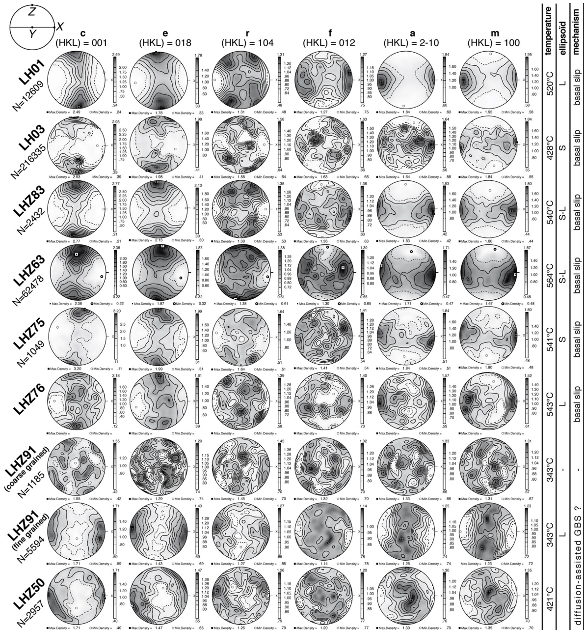
Fig. 5. Stereonets representing the Crystallographic Preferred Orientation (CPO) of calcite in mylonitic marbles from the Aulus basin. All samples display a well-defined although weak CPO. Temperatures are peak temperatures determined using the Raman spectroscopy of carbonaceous material (RSCM) as described in Clerc et al. (2015). Temperatures obtained from additional samples in the Aulus basin are reported in Fig. 1.
