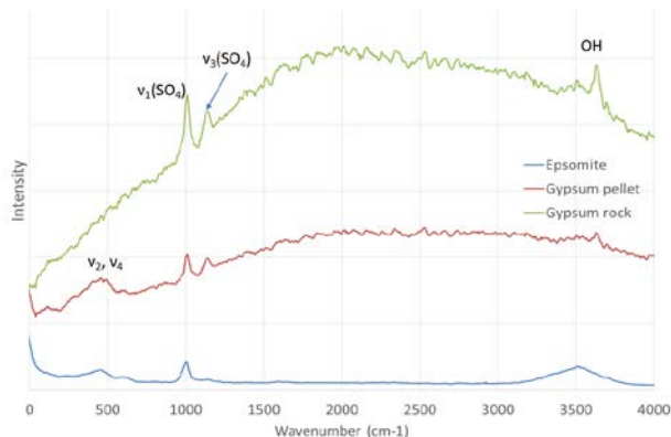
Fig. 3. Raman spectra from the SuperCam prototype transmission spectrometer. Spectra were obtained at 4 m distance using 1000 laser shots. The detector was exposed for a total of 100 s at room temperature to obtain these spectra. With the flight unit the CCD will be cooled and gated around the laser shots, greatly improving signal to noise.
