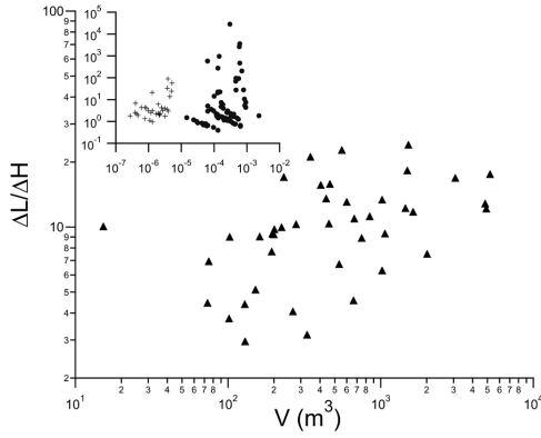
Figure 1. Mobility \Delta L/\Delta H of the Valles-Marineris Landslides as a function of their volume V . Data from Quantin et al. [2004]. Insert: same plot for the experimental collapses. Circles and crosses correspond to experimental data obtained respectively by Lajeunesse et al. [2004] in the axisymmetric geometry and by Lajeunesse et al. [2005] in a rectangular channel.
