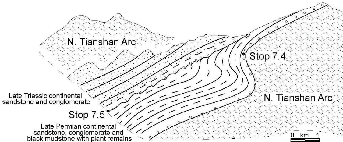
Figure 14. Schematic cross section of the Aiwegou section.
