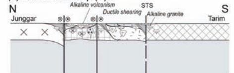
Figure 2. A tentative geodynamic model for the Paleozoic Chinese Tianshan (modified from Wang et al., 2008; Lin et al., 2009)
