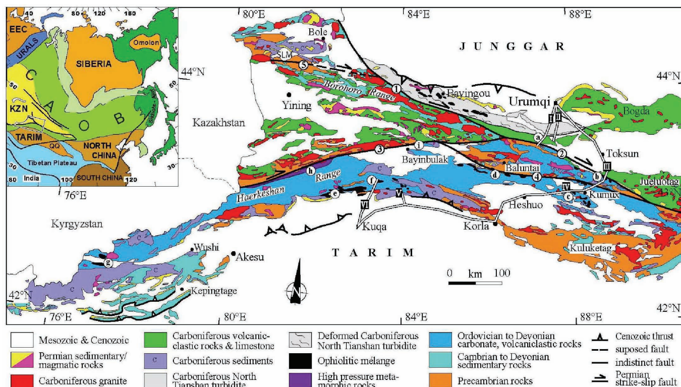
Figure 1. Geological map of the Chinese western Tianshan belt (modified after Wang et al., 2008). Numbers in circle refer to the main faults: 1-North Tianshan fault (NTF); 2-Main Tianshan shear zone (MTSZ); 3-Qingbulak-Nalati fault (QNF); 4-Sangshuyuanzi fault; 5-Jinghe fault. Letters correspond to localities cited in the text: a. Houxia; b. Gangou-Mishigou; c. Yushugou; d. Guluogou-Wuwamen; e. Heiyingshan; f. Kulehu; g. Aheqi; h. Kakesu; i. Nalati. Roman numbers stand for the excursion sections: I-Houxia section; II-Aiweiergou section; III-Gangou section; IV-Yushugou section; V-Cedaya section; VI-Duku road section. Inset shows location of the Tianshan Belt in Central Asia (modified from Jahn, 2004). Abbreviations: CAOB: Central Asian Orogenic Belt; EEC: Eastern European Craton; KZN: Kazakhstan; QQ: Qaidam-Qinling.
