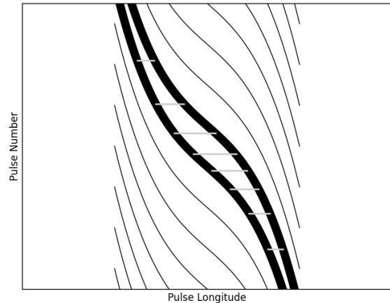
Fig. 1. Illustration of how curved driftbands mean that P_2 varies with pulse longitude. The black lines represent the shape of simulated driftbands. The grey lines represent the size of P_2 for the highlighted driftbands. One can see that P_2 varies significantly depending on the gradient of the driftbands at a given pulse longitude.
