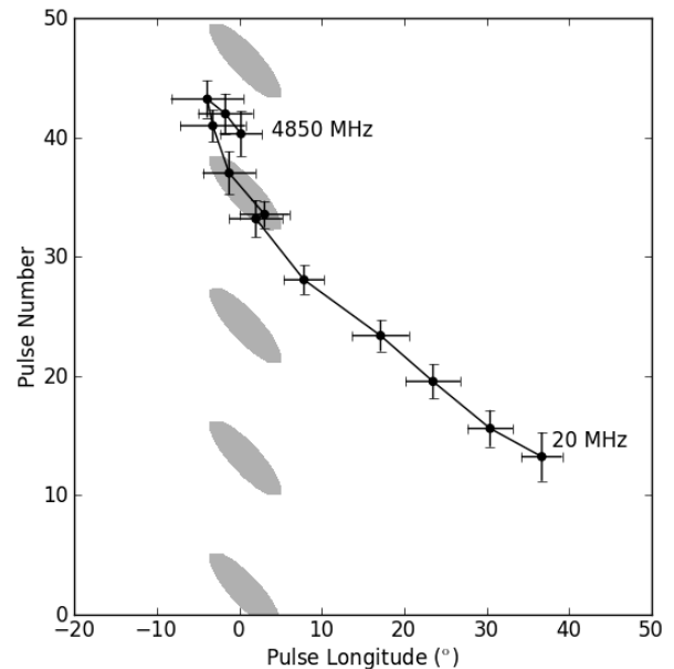
Fig. 6. The path of the moving driftband as a function of frequency. The shape of the stationary (“fiducial”) driftband corresponding to the fiducial pulse profile component is shown in grey.
