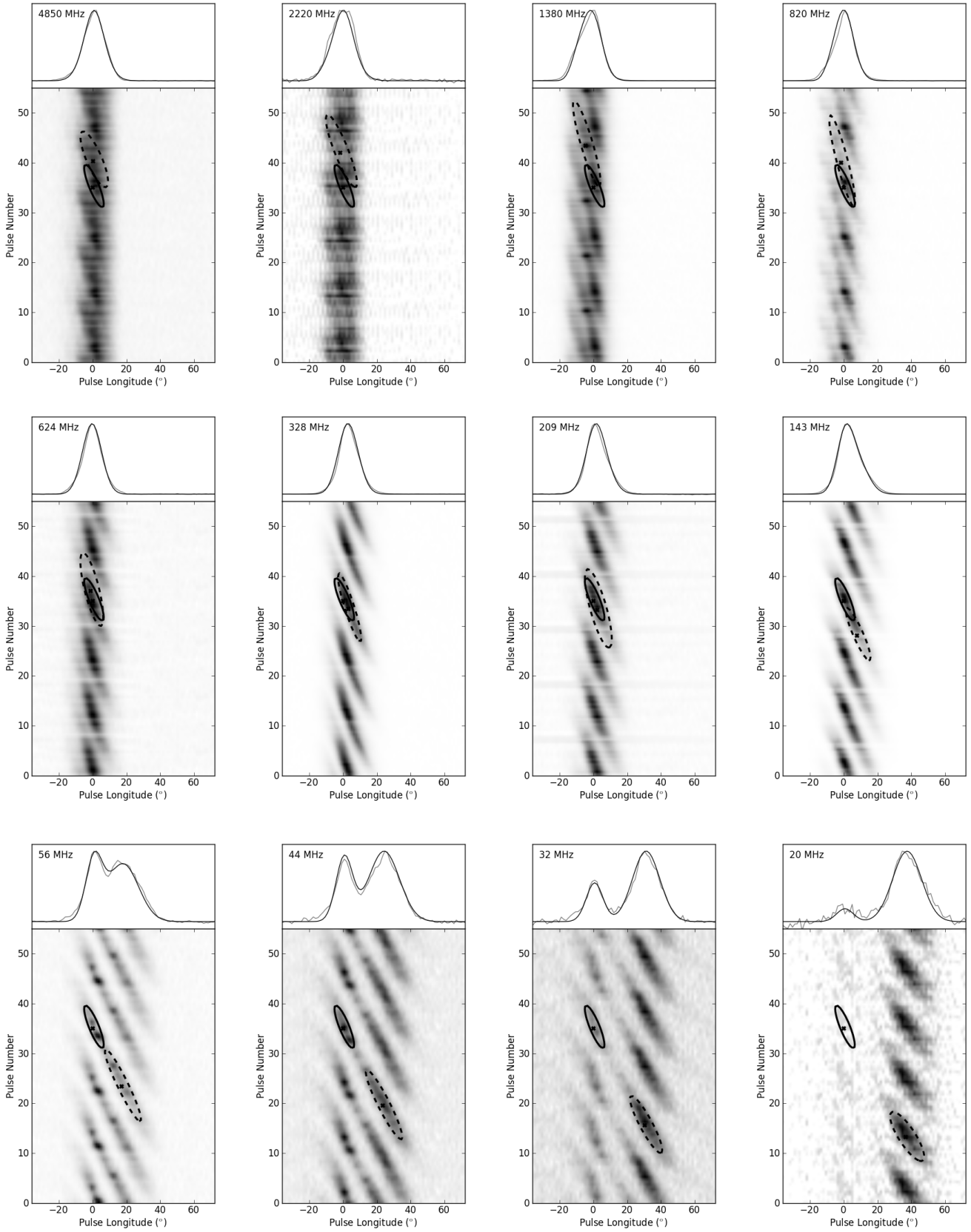
Fig. 5. Folded “pulse stacks” from each of the observations used. The solid and dashed ellipses show the half power points of 2D Gaussians fitted to the data using a least squares method. The central observing frequency of each panel is indicated in the top left corner. The driftbands are repeated over 5 \times P_3 so that the full drift pattern is visible at all frequencies. The pulse profile (grey line), and a simulated pulse profile (black line) from each 2D fit is shown in the panel above the corresponding pulse stack.
