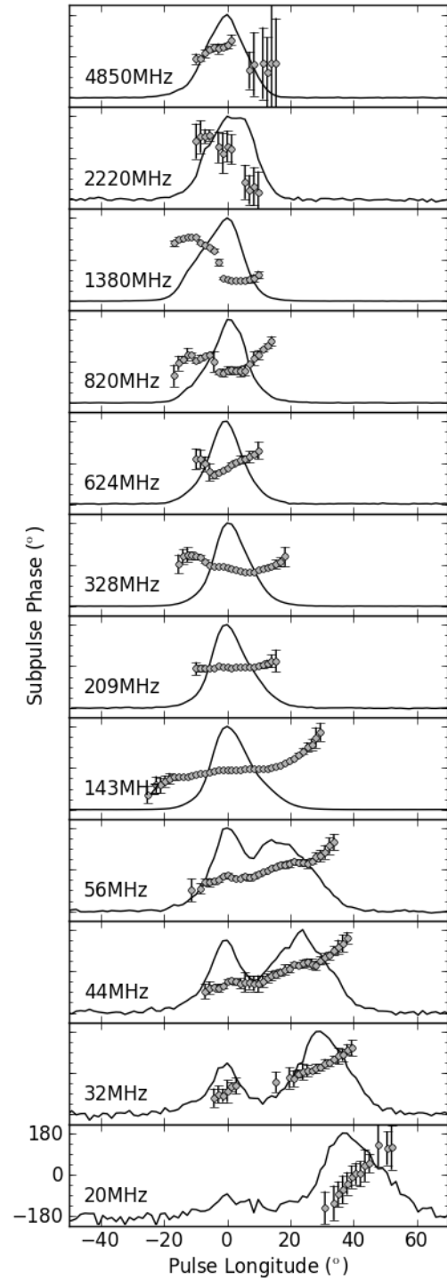
Fig. 4. The subpulse phase tracks (grey points) and average pulse profiles (black lines) of PSR B0809+74 between 14–5100 MHz. All phase tracks have had a constant slope of -25^\circ removed. The central observing frequency of each panel is indicated in the bottom left corner.
