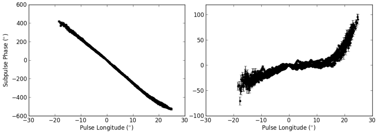
Fig. 3. The subpulse phase tracks of 8 \times 1.5 h blocks of a LOFAR HBA observation of PSR B0809+74, showing that the shape subpulse phase track remains approximately constant with time (typical spread is \sim 10^\circ ). The right panel shows the same tracks with a slope of -25^\circ/\circ subtracted, so that fine structure is easier to see.
