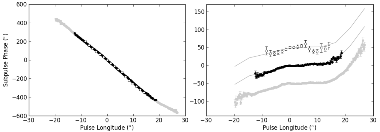
Fig. 2. The subpulse phase tracks of three LOFAR observations of PSR B0809+74 taken in March 2009 (white points), September 2009 (black points) and September 2011 (grey points). The right panel shows the same tracks with a slope of -25^\circ/\circ subtracted and offset by \pm 50^\circ , so that fine structure is easier to see. The grey line is a spline of the most recent observation so that data can be easily compared across epochs. The shape of the subpulse phase tracks are constant to within experimental uncertainties.
