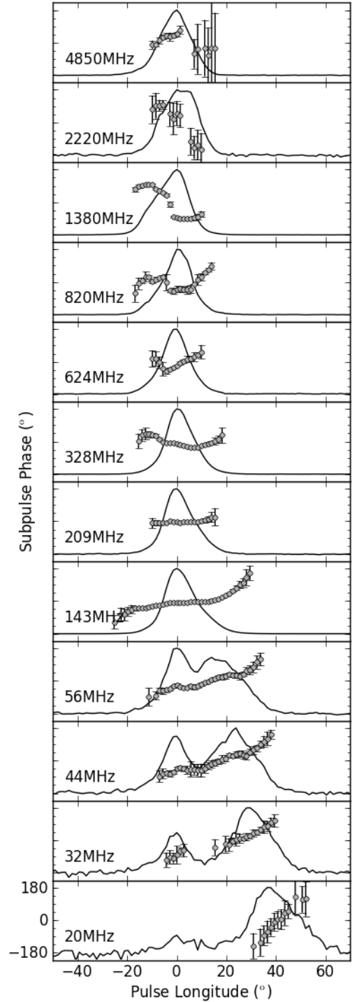
Fig. 4. The subpulse phase tracks (grey points) and average pulse profiles (black lines) of PSR B0809+74 between 14–5100 MHz. All phase tracks have had a constant slope of -25^\circ/\circ removed. The central observing frequency of each panel is indicated in the bottom left corner.
