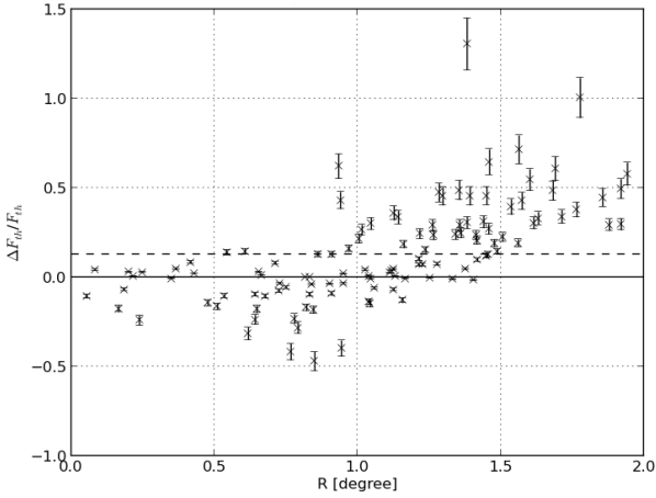
Fig. 6. The normalized peak flux differences between point sources in the LOFAR and WSRT observations as a function of radial distance. The LOFAR peak fluxes were rescaled to 150 MHz and both maps were corrected for primary beam attenuation. The mean value (dashed line) of these fractional variations is (\Delta F_p/F_p) = (0.128 \pm 0.014) , indicating the presence of a bias.
