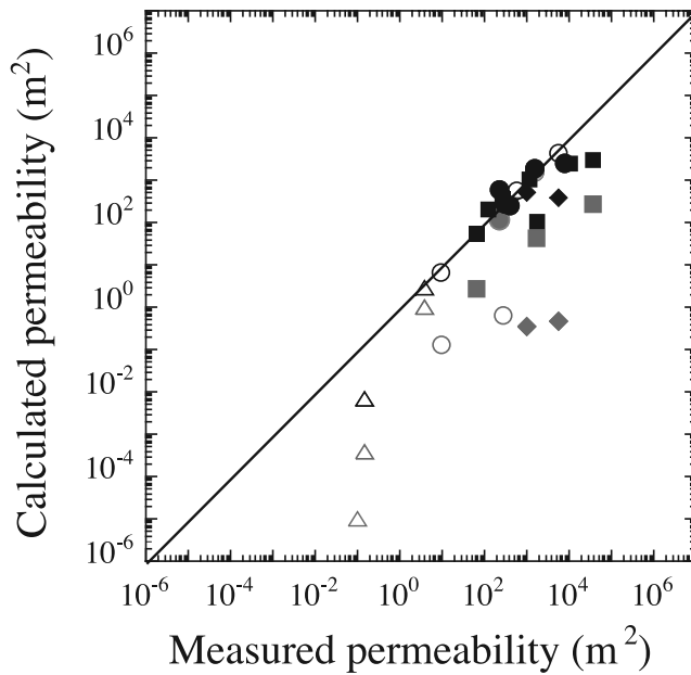
Figure 7. Comparison of measured permeability with the calculated values using the theoretical models of Carman-Kozeny [Carman, 1956] (gray symbols) and Katz and Thompson [1986, 1987] (black symbols).
