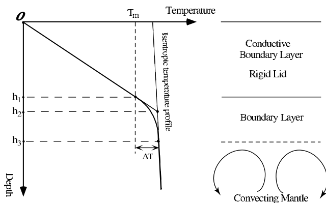
Figure 1. Thermal structure of the continental lithosphere and underlying mantle. The thickness of continental lithosphere can be defined in three different ways. The thickness of the purely conductive boundary layer, or rigid lid, is h_1 , which is the definition used here. h_2 is determined from the intersection of the conductive temperature profile and an assumed isentropic temperature profile in the convecting mantle. h_3 is the total thickness of the thermal boundary layer, defined as the layer where temperature departs significantly from the isentropic profile. Seismological studies provide constraints on h_2 or h_3 .
