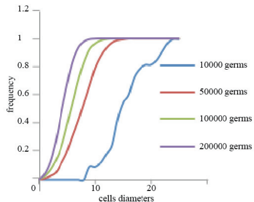
Figure 6. Comparison of size distribution of fragments having at least 80% of useful mineral. Cells diameters are in voxels (modified after Ngassa Tankeu 2014).
