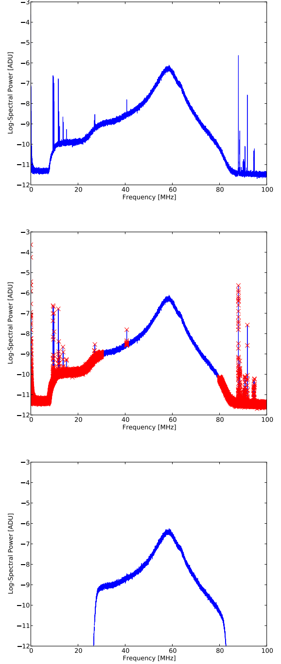
Fig. 6: The average spectrum of a typical LBA event. The raw data ( top ), with flagged contaminated channels ( middle ), cleaned and clipped to 30 – 80 MHz ( bottom ).
