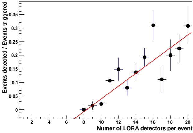
Fig. 21: Fraction of air showers with a detectable radio signal over the number of air showers triggered with a scintillator signal is plotted against the number of particle detectors above threshold in an event. The red straight line is a fit to the data.
