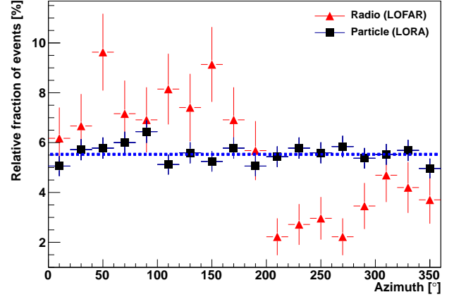
Fig. 24: Binned distribution of the azimuth angles of all events measured with the particle detectors (black squares) and those in coincidence of particle detectors and radio antennas (red triangles). The best fit of a straight line to the particle data is also shown. The fit has a \chi^2/\text{nDoF} = 0.9 .
