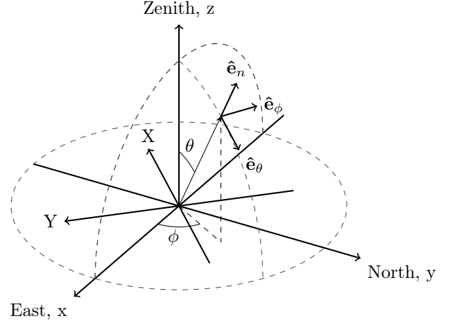
Fig. 13: On-sky polarization coordinate frame ( \hat{\mathbf{e}}_\theta , \hat{\mathbf{e}}_\phi , \hat{\mathbf{e}}_n ). Also depicted is the (north, east, zenith) coordinate frame of the simulations, where the unit vectors ( \hat{\mathbf{e}}_x , \hat{\mathbf{e}}_y , \hat{\mathbf{e}}_z ) correspond to the x , y and z -axis, respectively. Furthermore the dipole antennas X and Y are shown.
