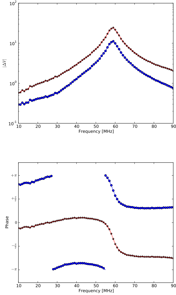
Fig. 14: Jones matrix components of the antenna model amplitudes ( top ) and phases ( bottom ) for a dipole receiving a wave polarized in the \hat{e}_\theta direction (circles) and a wave polarized in the \hat{e}_\phi direction (stars) for an arrival direction of \phi = 345^\circ, \theta = 50^\circ . Also plotted, as the dotted line, are the interpolated values.
