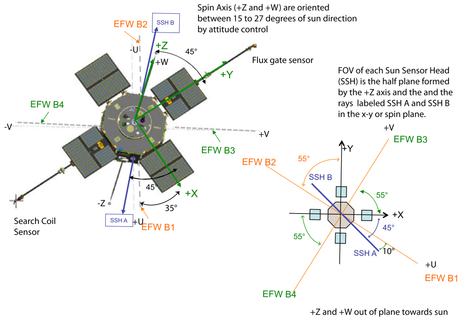
Fig. 7 Overview picture of RBSP spacecraft showing orientation of EFW spin plane boom sensors, EFW axial boom sensors, and EMFISIS 3-D Magnetic Search Coil sensors, spacecraft coordinates (xyz) and sensor coordinates (UVW) are indicated. Also shown are the two Sun Sensor Heads (SSH A and B) FOV directions relative to spacecraft coordinates and EFW spin plane booms. Magnetic Search Coil sensors directions and EFW booms are aligned in a common the UVW coordinate system for ease of analysis
