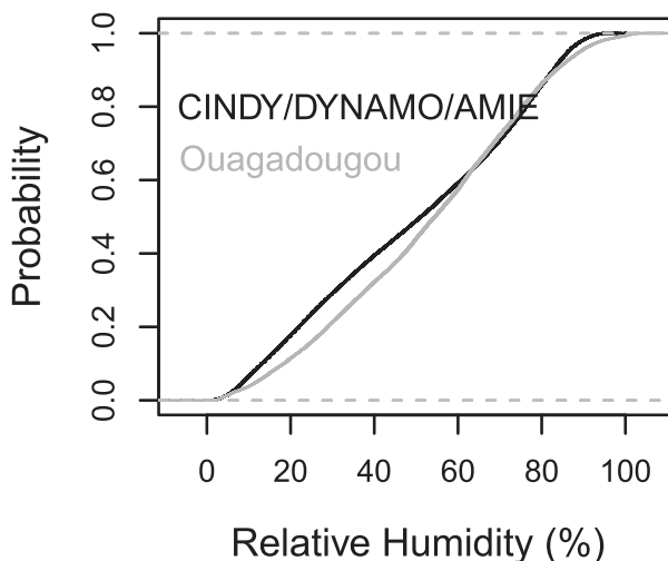
FIG. 1. Cumulative distribution functions of RH (%RH) within the CDA set (black curve) and within the Ouagadougou set (gray curve).
