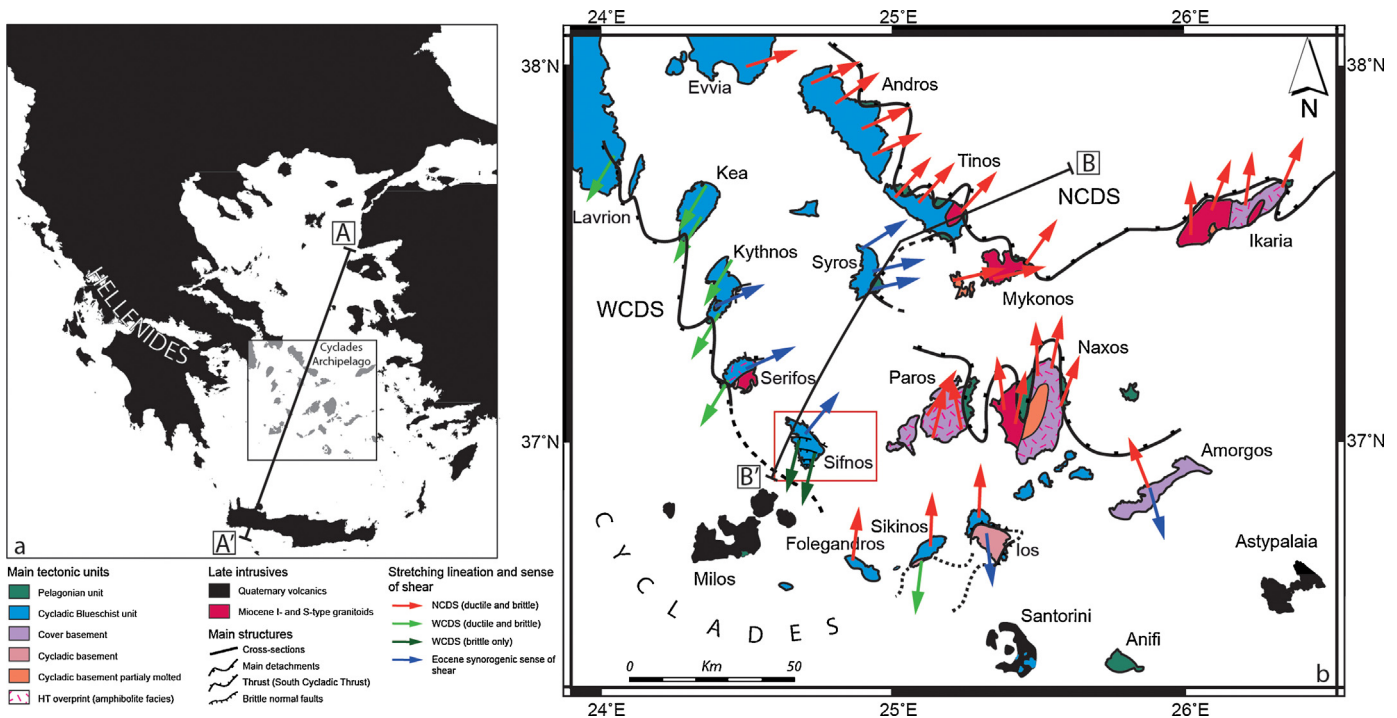
Fig. 1. Tectonic map of the Aegean domain. Tectonic map of the Aegean domain and schematic geological map of the Cyclades showing the main structures related to both syn-orogenic and post-orogenic episodes, modified after Jolivet and Brun (2010). The original map has been modified incorporating recent works (Kumerics et al., 2005; Rosenbaum et al., 2007; Huet et al., 2009; Grasmann et al., 2012; Augier et al., 2015; Laurent et al., 2015; Beaudoin et al., 2015). Stretching-parallel cross-section through Aegean domain (Fig. 1a) and central Aegean (Fig. 1b) are indicated. Red box: Location of Sifnos. (For interpretation of the references to colour in this figure legend, the reader is referred to the web version of this article.)
