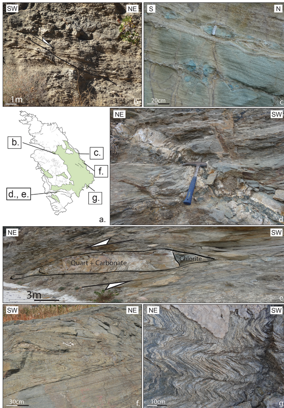
Fig. 10. Macrostructures observed in Faros Unit (FU). (a) Location of field photographs. (b) S-C Structures with top-to-the-NE sense of shear characterized by metric shear bands in a metapelite. (c) Asymmetric mafic eclogite boudins cross cut by quartz-carbonate veins showing a north-south stretching. (d) Sheared quartz-carbonate veins cross cut the main foliation and (e) are commonly transposed in the foliation with pressure shadows filled in chlorite and albite showing top-to-the-NE sense of shear. (f) Centimetric folds showing axes mostly perpendicular to the stretching direction. (g) Axial plane crenulation cleavage associated with the hinge of folds at the base of this unit.
