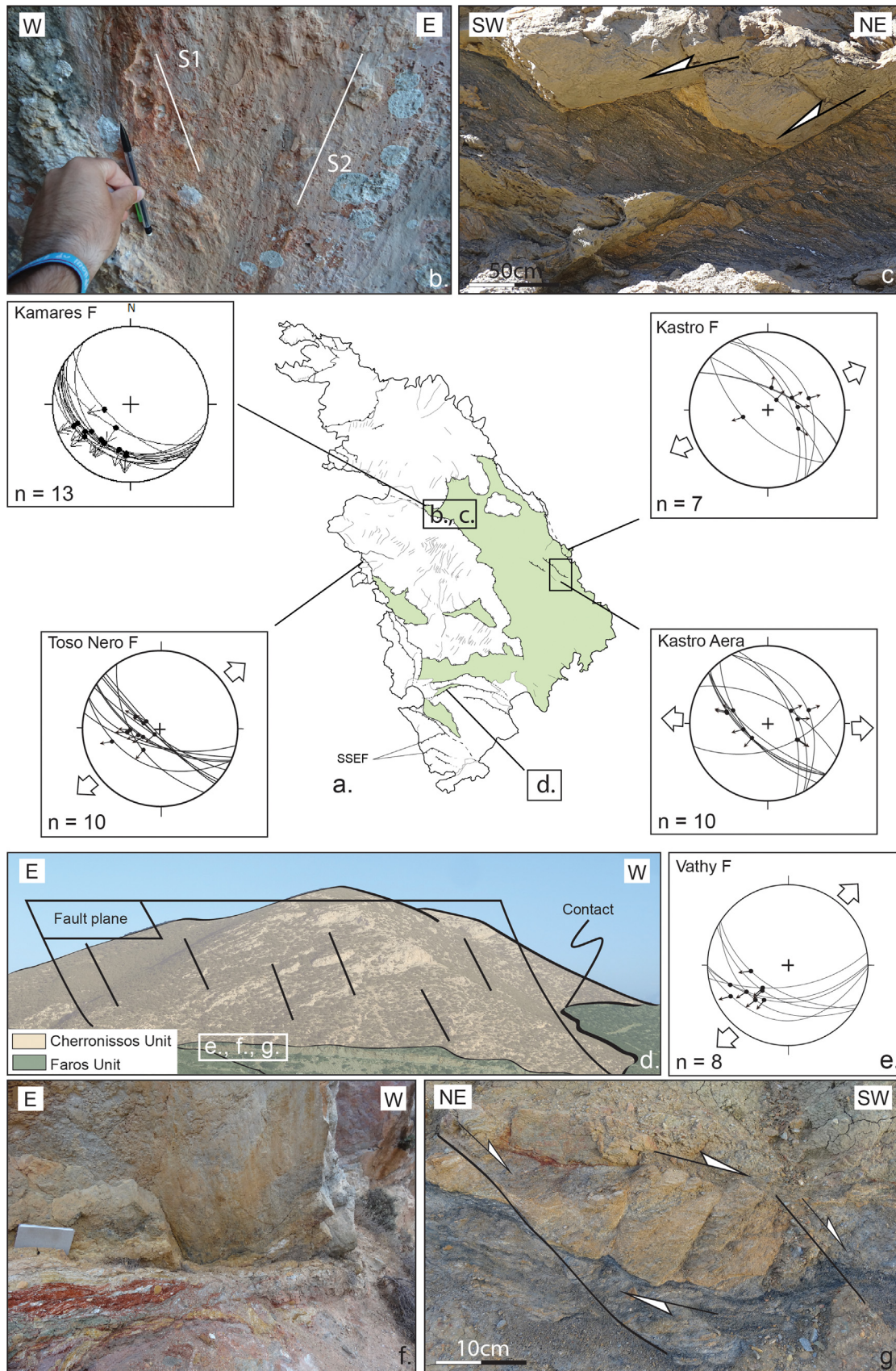
Fig. 5. Brittle deformation on Sifnos. (a) Location of fault-slip data from high-angle normal faults. The diagrams show great circles of fault planes and the projected trace of slickenside lineations in a lower hemisphere equal-area projection. Arrows indicate extension directions from the measured fault sets (paleostress orientation patterns were calculated with the win-tensor computer-aided inversion software of Delvaux and Sperner, 2003). Readers unfamiliar with the method, or more generally with fault-slip data inversion are referred to the work of Angelier (1990). (b) Kamares Fault showing two slicken-fibre generations. (c) Top-to-the-SW brittle-ductile kinematic indicators associated with Kamares Fault. (d) Vathy SW dipping normal fault with (e) stereographic projections of striations. (f) Fault plane characterized by a few meters thick reddish fault gouge showing (g) top-to-the-SW brittle-ductile kinematic indicators. Note the consistency of the NNE-SSW to E-W direction of brittle extension all over the island.
