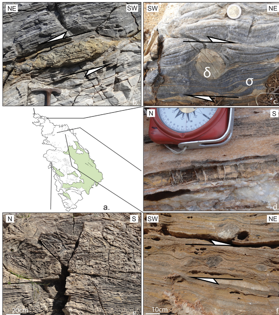
Fig. 9. Microstructures and macrostructures observed in Upper Marble Complex and Main Marble Unit. (a) Location of field photographs. (b) Difference of competence between calcite and dolomite showing the development of dominos and (c) delta/sigma clasts indicating top-to-the-NE sense of shear. (d) North-south stretching shown by calcite recrystallization within tension gashes. (e) Centimetric folds showing axes mostly perpendicular to the stretching direction. (f) Top-to-the-NE shear sense defined by the asymmetric shape of stretched carbonate pebbles in metaconglomerate layers.
