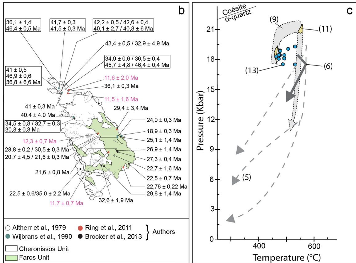
Fig. 3. P-T conditions and deformation ages within Cheronissos and Faros units. (a) Geological pile on Sifnos showing different ages of metamorphic peak conditions, and blueschist-facies (BS) to greenschist-facies transition (GS) with the associated depths. Superscript numbers indicate the citations, 1) Altherr et al., 1979; 2) Schliestedt and Matthews, 1987; 3) Wijbrans et al., 1990; 4) Avigad et al., 1992; 5) Trotet et al., 2001a; 6) Schmadicke and Will, 2003; 7) Forster and Lister, 2005; 8) Spear et al., 2006; 9) Groppo et al., 2009; 10) Ring et al., 2011; 11) Dragovic et al., 2012; 12) Bröcker et al., 2013; 13) Ashley et al., 2014. (b) Compilation of results of K-Ar, ^{40}\text{Ar}/^{39}\text{Ar} and Rb-Sr ages on phengite, paragonite and fission track on zircon. (c) Detailed P-T path modified after Ashley et al. (2014), subscript numbers indicate the References. (For interpretation of the references to colour in this figure legend, the reader is referred to the web version of this article.)
