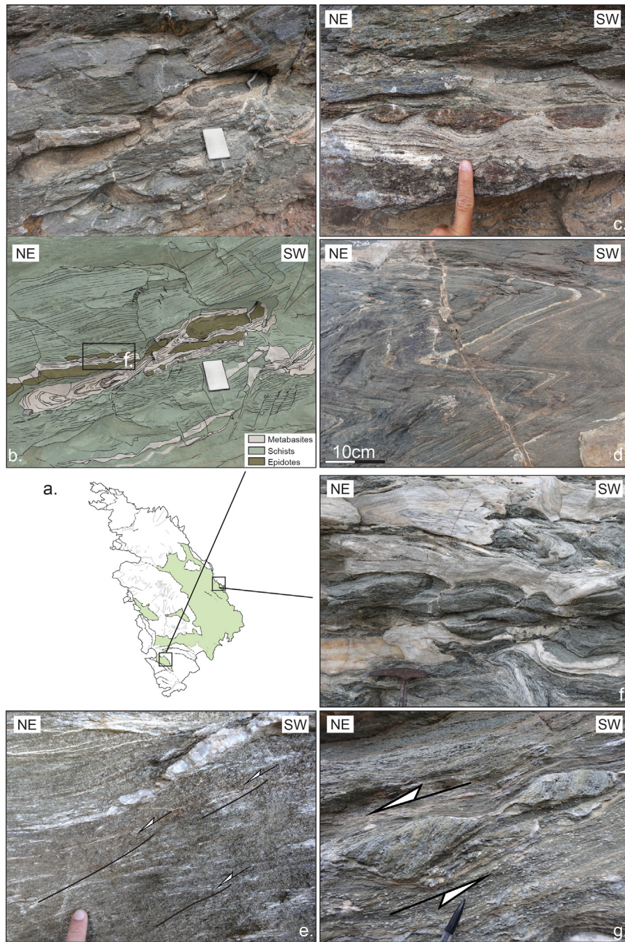
Fig. 12. COF contact. The COF contact is well exposed (a) Intense ductile deformation shown by folding in all lithologies. Top-to-the-NE shear bands associated with glaucophane affect the foliation. (b) Asymmetric boudinage of epidotite boudins showing a top-to-the-NE shear sense. (c) Closely-spaced shear bands associated with white mica indicate top-to-the-NE sense of shear close to Vathy. (d) Similar features observed close to Kastro, just below the main contact.
