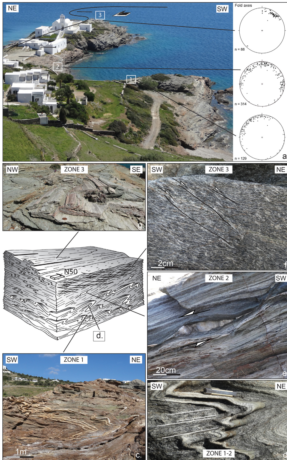
Fig. 11. Chryssopigi shear zone defined by a distinct gradient of shearing deformation. (a) Large scale representative view of the Chryssopigi shear zone in the south-eastern part of the island. Albite pods marked the stretching lineation trending N50°E. All information is summarized with synthetic 3-D diagrams. This shear zone is divided in three areas; zone 1 corresponds to (c) an intense folding and (a) associated Schmidt's lower hemisphere equal-area projections showing fold axes dispersion; zone 2 is defined by (d) axial plane crenulation cleavage associated with the hinge of folds. (a) Fold axes tend to progressively rotate toward the shearing direction. (e) Sheared lenses of quartz and calcite showing a top-to-the-NE sense of shear; zone 3 is marked by intense non-coaxial shearing consistent with an overall top-to-the-NE kinematics. (f) Shear bands spacing ranges from few millimetres and (g) a-folds are commonly observed. Note that folds axes are now parallel to the stretching direction.
