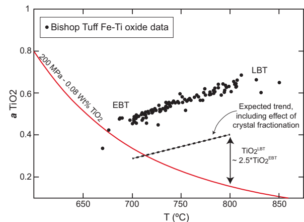
FIGURE 7. Curve of aTiO_2 vs. T at 200 MPa for a Bishop Tuff composition with 0.08 wt% TiO_2 and corresponding loci of the Fe-Ti oxides (dots), from Ghiorso and Gualda (2013) with permission of Springer, compared to the expected change in aTiO_2 vs. T (dashed line) assuming a difference of X2.5 in melt TiO_2 between EBT at 700 °C and LBT at 800 °C (see text for details).
