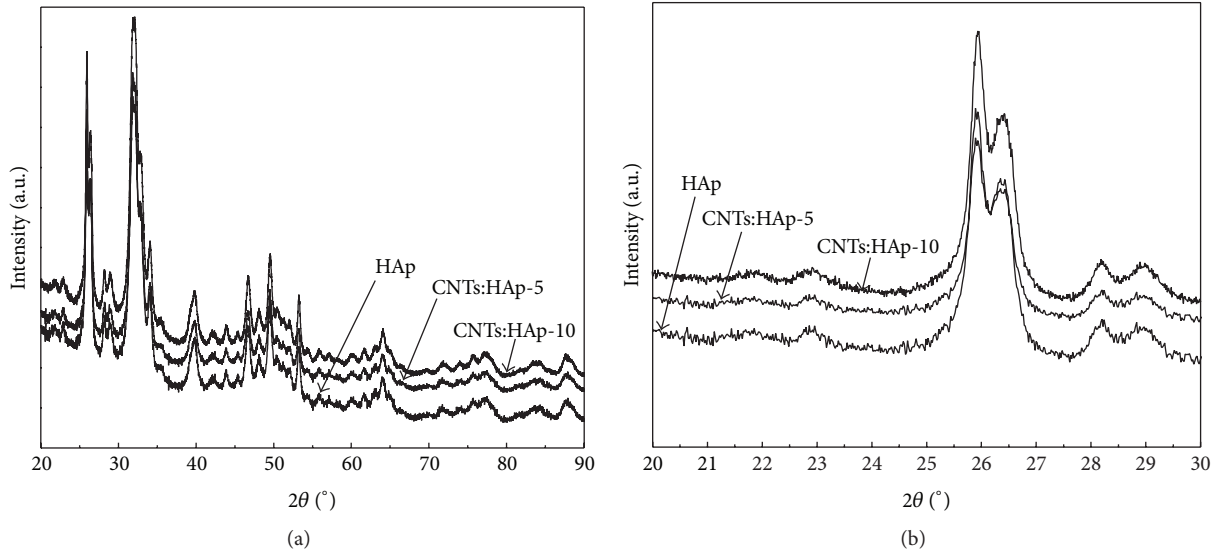
FIGURE 1: Comparative representation of the experimental XRD patterns of the HAp and CNTs:HAp-5 and CNTs:HAp-10 nanocomposites in the 2\theta ranges 20^{\circ} – 90^{\circ} (a) and 20^{\circ} – 30^{\circ} (b), respectively.
