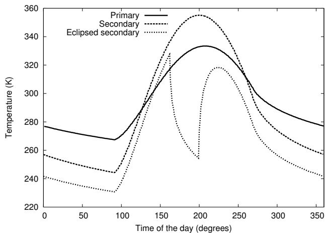
Figure 6: Equatorial temperatures as a function of time of day (measured in degrees) at the perihelion distance ( q \sim 1.01338 \text{ AU} ) for the primary, Didymoon, and for an area on Didymoon subject to solar eclipses caused by the primary. This area is located at the “sub-primary” point of Didymoon, i.e., at the point on Didymoon’s surface closest to the primary. Local noon occurs at 180 degrees. The bold dashed curve is for the far (unc eclipsed) side of Didymoon and the thin dashed curve is for its near (eclipsed) side. The bolometric Bond albedo is calculated to be 0.059, resulting from the geometric visible albedo of 0.15 and an assumed G-value of 0.15.
