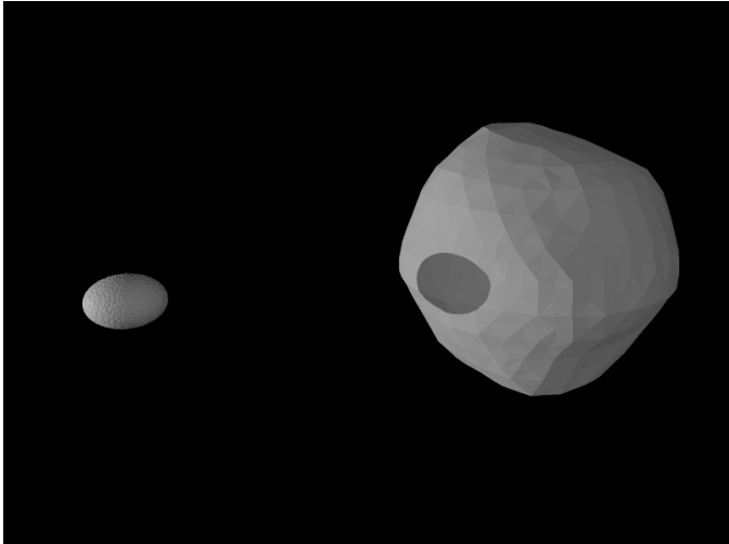
Figure 4: Preliminary shape model of the primary of Didymos obtained from combined modeling of the radar and photometry data from 2003, shown with Didymoon at scale with assumed ellipsoid axes (see Table 5).
