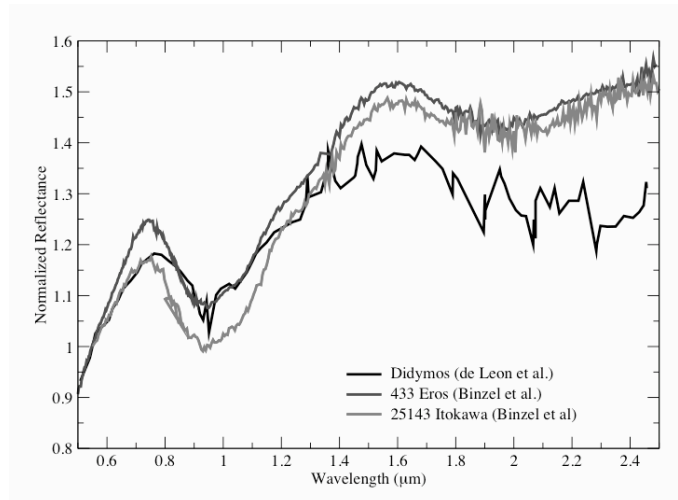
Figure 5: Spectrum of Didymos (de León et al., 2010), compared with that of two other S-types, namely Eros and Itokawa.
