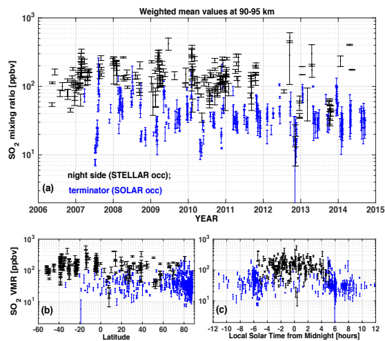
Fig. 3. Time (a), latitude (b) and Local time (c) diagrams of SO 2 variations at altitude level 90-95 km (blue – solar occultations, black – stellar occultations).
