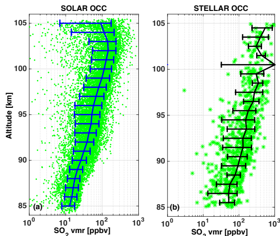
Fig. 2. Altitude distribution of SO 2 mixing ratio from SPICAV UV solar (a) and stellar (b) occultations. Solid lines are weighted mean values with standard deviations. Error bars of individual dots (not shown) are less than the dispersion of the data.
