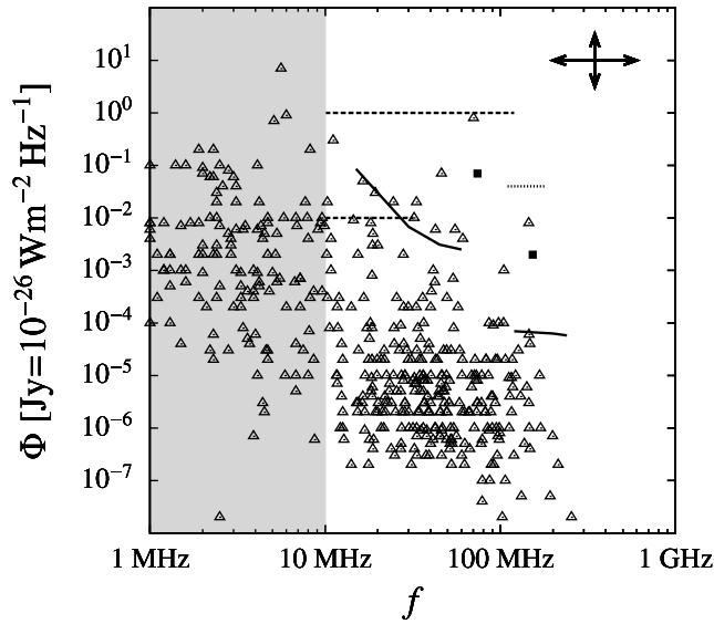
Figure 1. Maximum emission frequency and expected radio flux for known extrasolar planets for a rotation-dependent planetary magnetic field (adapted and updated from Griessmeier et al. [2007b]). Open triangles, predictions for planets. For comparison, the approximate sensitivity of the arrays described in the text is shown (for 1 h of integration time and a bandwidth of 4 MHz, or an equivalent combination): the upgraded UTR-2 (lower dashed line), the NDA (upper dashed line), the VLA (upper solid square), the WSRT (fine dotted line), the GMRT (lower solid square), LOFAR (two dash-dotted lines, one for the low band and one for the high band antenna). Frequencies below 10 MHz are not observable from the ground (ionospheric cutoff).
