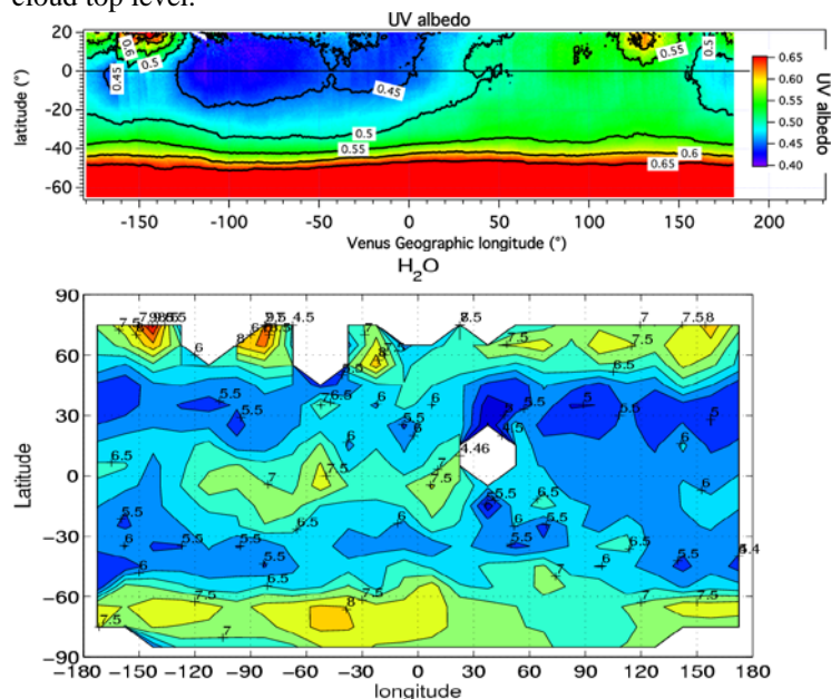
Figure 5a top. Venus geographic map of the UV albedo. The number of points per bin ranges from ~1000 to 5000. Iso-contours of UV albedo are drawn.
