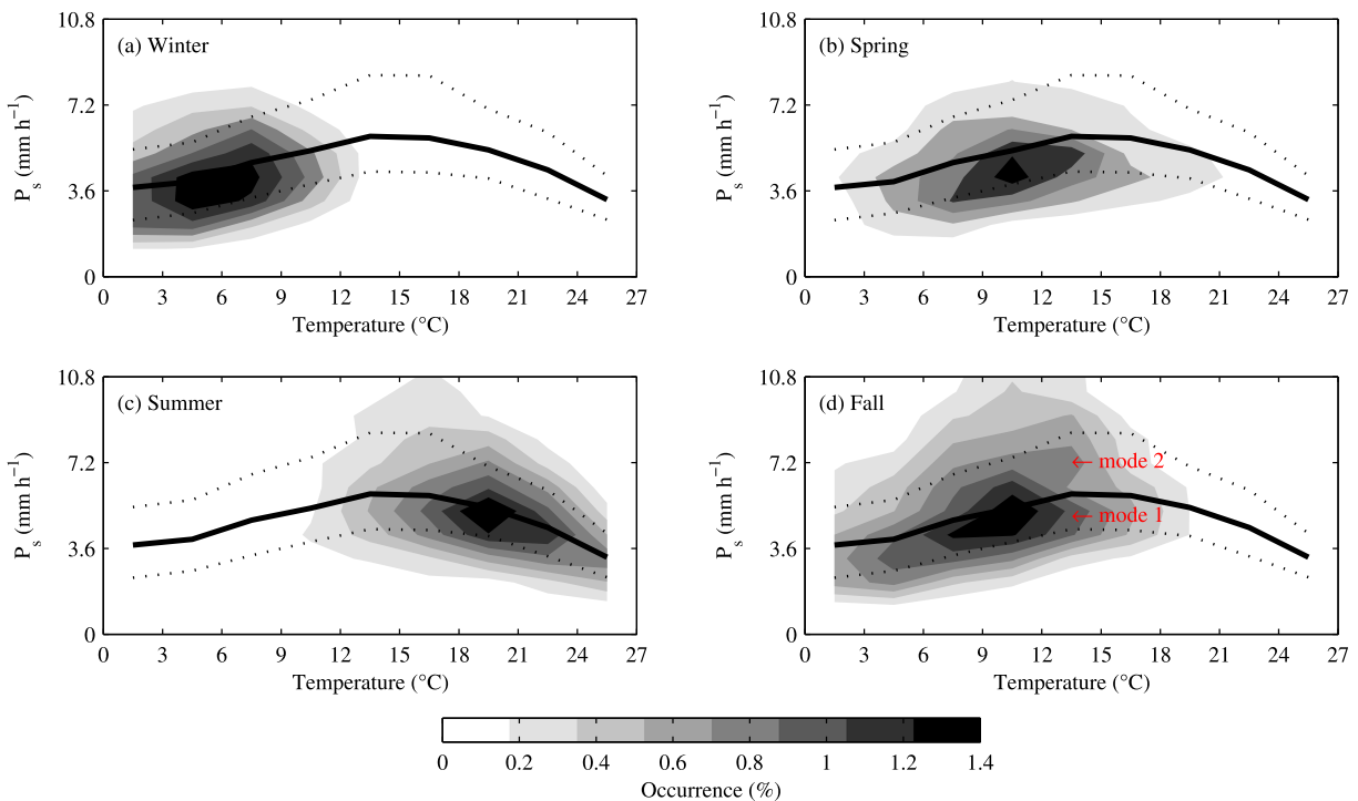
Figure 11. Occurrence of extreme precipitation computed from the WRF simulations as a function of daily temperature and 3-hourly precipitation intensity in (a) winter (January–March), (b) spring (April–June), (c) summer (July–September), and (d) fall (October–December). The thick lines and dotted lines correspond to the ensemble average and the 20th and 80th percentiles of precipitation extremes, respectively (see Figure 3).
