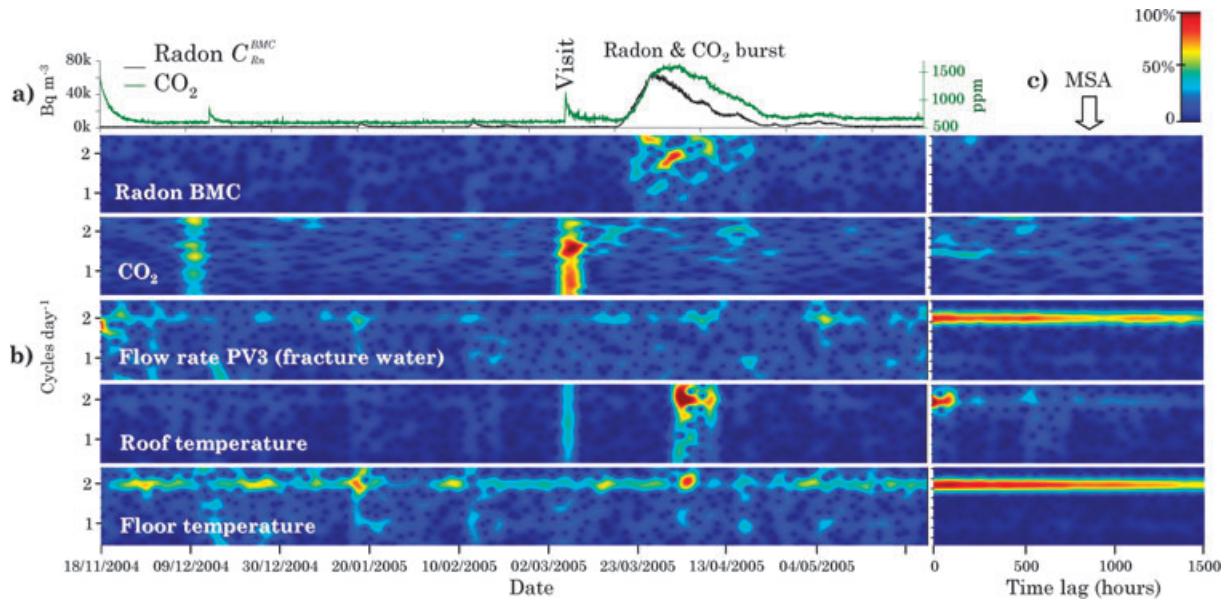
Figure 10. Spectral analysis of CO_2 , radon (BMC), fracture water flow rate, floor and roof temperature in the Roselend tunnel during Period 2 (see Fig. 3). (a) Radon and CO_2 time-series. (b) Classical spectrograms as a function of time. (c) MSA applied to each parameter.
