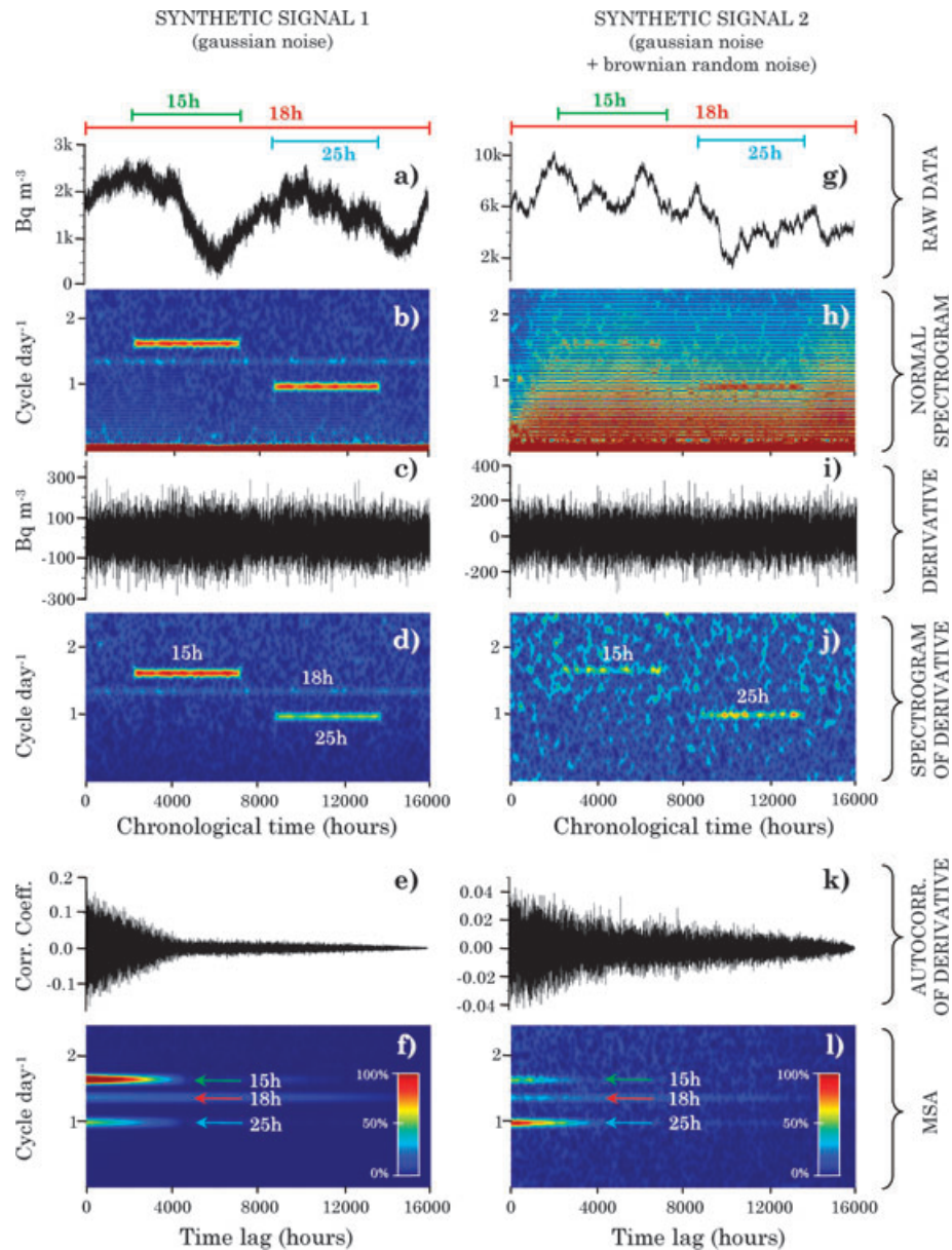
Figure 1. Modified Spectrogram Analysis (MSA) protocol (a–f and g–l) applied on two different hourly synthetic signals: synthetic signal 1 (a), containing random noise, yearly variation and three frequencies (15, 18 and 25 hr) plus an annual cycle and synthetic signal 2 (g) containing a Brownian and Gaussian white noise, three frequencies (15, 18 and 25 hr) plus an annual cycle.
