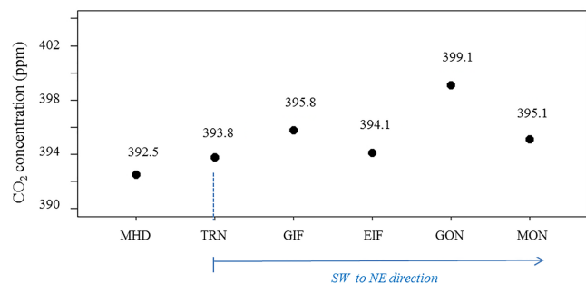
Figure 10. Mean CO 2 concentration (in ppm) observed at the different stations of the Paris regional network (TRN represents the measurements at 50 m a.g.l.) and at MHD for wind speed higher than 9 \text{ m s}^{-1} over the period of study (8 August 2010–13 July 2011). During such events, the synoptic conditions were mostly oceanic (wind blowing from the SW sector). Note (in m a.g.l.): MON is at 9 m (NE rural site), GON is at 4 m (NE peri-urban site), EIF is at 317 m (urban site), GIF is at 7 m (SW peri-urban site), TRN50 is at 50 m (SW rural site), TRN180 is at 180 m (SW rural site) and MHD is at 15 m (remote site).
