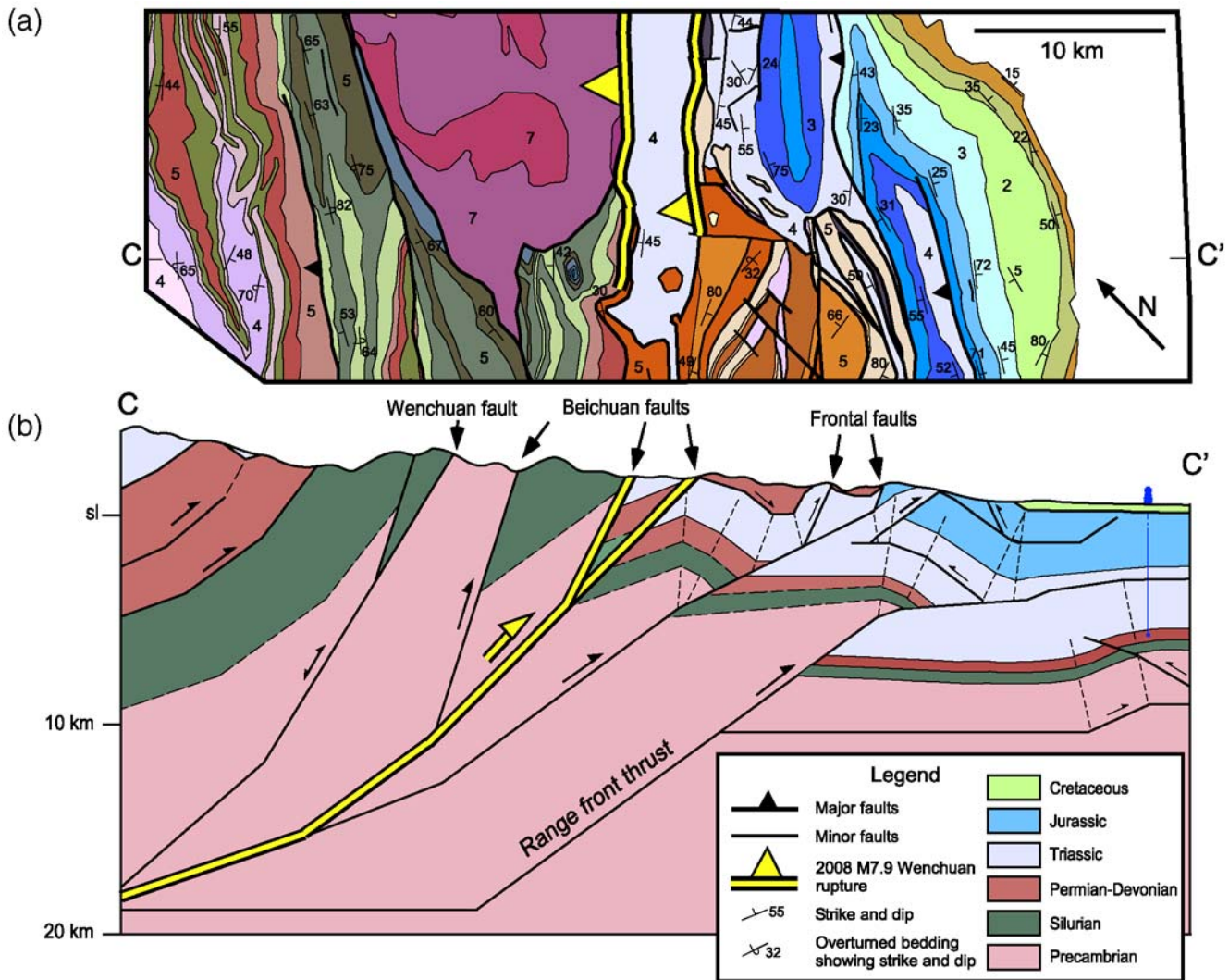
Figure 7. (a) Strip of geological map showing the surface data used to constrain cross section C-C' (see Fig. 2 for full map). (b) Cross section C-C', shaded to roughly correspond to the map. Note that the right side of the cross section is further constrained by the seismic data shown in Figure 5. The shades and numbers in the strip map are the same as in Figure 2. The Beichuan fault splits into several splays in this location, of which two ruptured. The color version of this figure is available only in the electronic edition.
