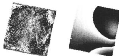
Figure 4. Measured and best fitted interferograms over zone 1. Projection vector (0.38; -0.08; 0.92). Average deformations are consistent but further interpretation is not reasonable due to low amplitude of observed and modeled deformation compared to the noise in the interferogram.
