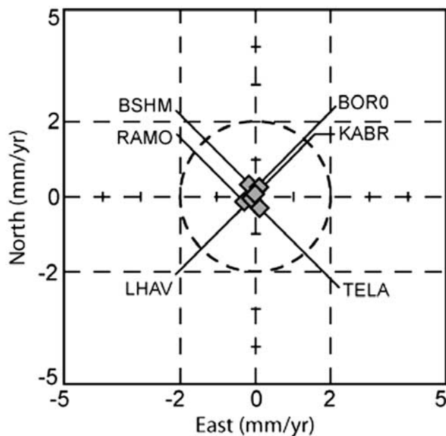
Figure 7. Residual velocities relative to Sinai for the sites used to determine the Sinai block Euler vector in ITRF2000.
