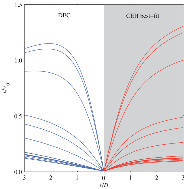
Figure 7. Comparison between velocity profiles from a DEC (blue lines, left side) model and corresponding best-fit profiles assuming a CEH (red lines, right side) space model. The CEH lines are meant to show how the CEH model may often approximate a DEC model in the near field (within three locking depths of the fault). Throughout we assume that geodetically constrained fault slip rates are estimated by this mapping from DEC to best-fitting CEH model. The disagreement between the two models is greatest at the beginning of each earthquake cycle.
